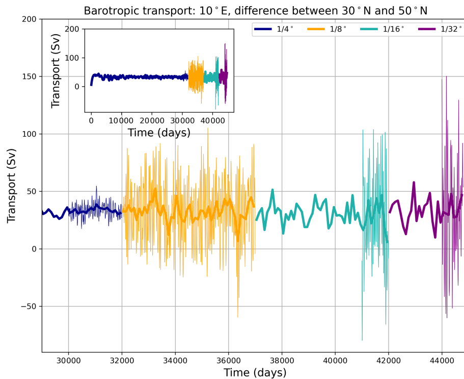
Figure 5. Time series of the difference in the barotropic transport stream function at 10^{\circ} E between 30^{\circ} N and 50^{\circ} N for each of the model horizontal grids during spinup and equilibration. Thin lines are 5 d means (where available), and thicker lines are 100 d means. The inset shows the entire time series, which starts from the 1/4^{\circ} configuration at rest.
