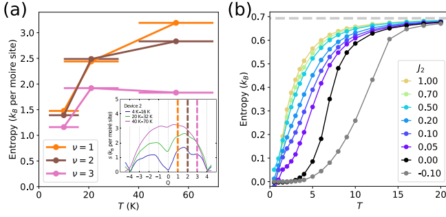
FIG. 4. (a) Entropy vs temperature T at various integer fillings of MATBG adapted from Ref. [50]. Inset: Original figure presented in Ref. [50], with vertical cuts illustrating how the data was adapted for the main figure. (b) Entropy vs temperature for various values of J_2 in our model (3). Dashed line at the value of S = \ln 2 indicates the extrapolated zero-temperature residual entropy.
