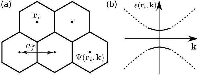
FIG. 2. (a) We coarse-grain our system into hexagonal regions centered at \mathbf{r}_i of size a_f that form a triangular lattice. In the mean-field model (2), the Ising order-parameter \mathcal{O}(\mathbf{r}_i) takes values \pm 1 on each hexagonal plaquette. (b) Spectrum \varepsilon(\mathbf{r}_i, \mathbf{k}) near the Dirac points that have been gapped by interaction-induced symmetry breaking. Higher momentum fermions \Psi(\mathbf{r}_i, \mathbf{k}) in these regions are integrated out, leaving a mean field model for the modes near \mathbf{k} = 0 .
