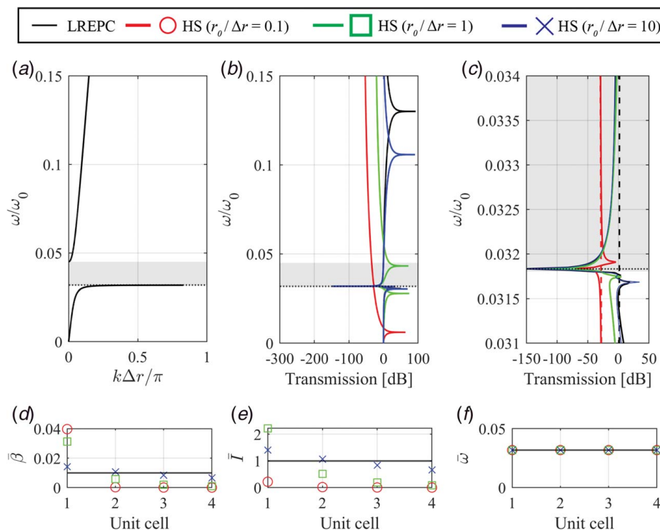
Fig. 5 (a) LREPC band structure, (b) transmission, (c) zoom in of transmission close to the lower band gap edge, (d) \bar{\beta} , (e) \bar{I} , and (f) \bar{\omega} for each unit cell. Black-dotted lines indicate the resonance frequency of the LREPC and HS resonators. Dashed lines on (c) represent the response of the LREPC and HS system with rigidly attached resonators. For clarity, these are plotted only for the LREPC and the HS with the lower r_0/\Delta r .
