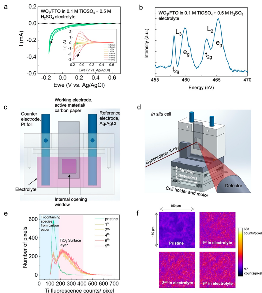
Figure 1. Formation of the amorphous \text{TiO}_2 surface layer on the \text{WO}_3 electrode surface. (a) Cyclic voltammetry (CV) of the \text{WO}_3/\text{FTO} electrode for 3 CV cycles in the 0.1 M \text{TiOSO}_4 + 0.5 M \text{H}_2\text{SO}_4 electrolyte at 0.1 mV/s scan rate with -0.165 V– 0.635 V vs Ag/AgCl (3M, NaCl). The inset is the CV curves of the \text{WO}_3/\text{FTO} electrode in the 0.1 M \text{TiOSO}_4 + 0.5 M \text{H}_2\text{SO}_4 electrolyte at various scan rates within the same potential range. The arrow indicates the direction of CV cycling. (b) Ti L-edge s-XAS in the TEY (total electron yield) mode of the \text{WO}_3/\text{FTO} electrode after 3 CV cycles in the 0.1 M \text{TiOSO}_4 + 0.5 M \text{H}_2\text{SO}_4 electrolyte at 0.1 mV/s scan rate with -0.165 – 0.635 V vs Ag/AgCl (3M, NaCl). No pre-edge features, no splitting of the \text{L}_{3\text{-e}_g} subband, and the higher peak intensity of the \text{L}_{3\text{-e}_g} subband (compared to the \text{L}_{3\text{-t}_{2g}} subband) suggest the amorphous feature of \text{TiO}_2 . Only the TEY mode is analyzed in s-XAS because the thin thickness of the newly formed \text{TiO}_2 surface layer gives the FY (fluorescence yield) mode a relatively noisier signal. (c) The specific structure of the in situ XFM electrochemical cell is a three-electrode electrochemical system. Carbon paper is used as the substrate for better X-ray penetration. (d) In situ XFM experimental setup in the 2 ID-E beamline at the Advanced Photon Source. More details are in the experimental section. (e) Ti elemental distribution curves of the Ti-element fluorescence counts/pixel (pixel size: 1\ \mu\text{m} \times 1\ \mu\text{m} , X-axis) and the number of pixels (Y-axis) of the \text{WO}_3/\text{C} electrode during 3 CV cycles in the 0.1 M \text{TiOSO}_4 + 0.5 M \text{H}_2\text{SO}_4 electrolyte at 0.5 mV/s scan rate with -0.165 – 0.635 V vs Ag/AgCl (3M, NaCl). Pristine Ti elemental distribution curve is without the electrolyte, suggesting the existence of Ti-containing species from carbon paper. The 1st Ti elemental distribution curve is the one right after adding 0.1 M \text{TiOSO}_4 + 0.5 M \text{H}_2\text{SO}_4 electrolyte, indicating the beginning of slow electrochemical cycling. The subsequent 2nd to the 9th Ti elemental distribution curves show the evolution of Ti elemental distribution during the formation of the \text{TiO}_2 surface layer. (f) Ti-element XFM images during the formation of the \text{TiO}_2 surface layer in panel e, where the color bar on the right represents the absolute Ti-element fluorescence counts in each pixel.
