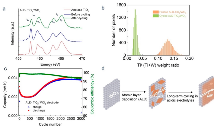
Figure 3. Structural evolution of ALD-made \text{TiO}_2 surface coating. (a) Ti L-edge s-XAS in the TEY (total electron yield) mode of the ALD-made \text{TiO}_2/\text{WO}_3 electrode before and after 3000 CV cycling in 0.5 M \text{H}_2\text{SO}_4 electrolyte at 60 mV/s scan rate with -0.165 – 0.635 V vs Ag/AgCl (3M, NaCl). (b) Ex situ XFM quantitative analysis of Ti/(Ti + W) weight ratio of the ALD-made \text{TiO}_2/\text{WO}_3 electrode before and after 3000 CV cycling. (c) The electrochemical capacity evolution of the ALD-made \text{TiO}_2/\text{WO}_3 electrode during the 3000 CV cycling. (d) Schematic illustration of the structural evolution of the ALD-made \text{TiO}_2 surface layer during electrochemical cycling: from crystalline to amorphous phase transformation and progressively uniform element distribution.
