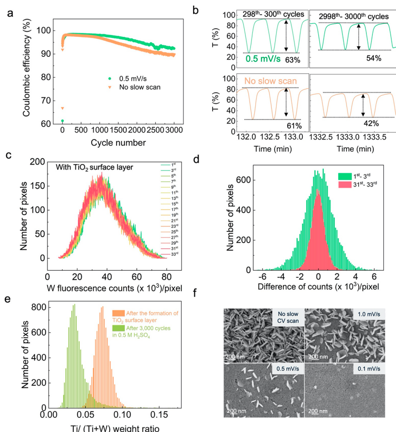
Figure 2. Alleviated dissolution of the WO 3 electrode after the formation of the amorphous TiO 2 surface layer. (a) Coulombic efficiency of the WO 3 /FTO electrode during 3000 CV cycles in 0.5 M H 2 SO 4 electrolyte at 60 mV/s scan rate with −0.165–0.635 V vs Ag/AgCl (3M, NaCl). 0.5 mV/s refers to the formation of an amorphous TiO 2 surface layer with 0.5 mV/s slow scan in 0.1 M TiOSO 4 + 0.5 M H 2 SO 4 electrolyte. No slow-scan refers to the controlled sample without the TiO 2 surface layer. (b) Optical modulation of the WO 3 /FTO electrode during 3000 CV cycles. (c) W elemental distribution curves of the W-element fluorescence counts/pixel (pixel size = 1 μm × 1 μm, X-axis) and the number of pixels (Y-axis) during 3000 CV cycling in the 0.5 M H 2 SO 4 electrolyte at 60 mV/s scan rate with −0.165–0.635 V vs Ag/AgCl (3M, NaCl). The total image size is 150 μm × 110 μm with a total of 16 500 pixels. The 1st W elemental distribution curve is the first one during 3000 CV cycling. (d) Quantitative analysis of the evolution of local W content in each pixel with the TiO 2 surface layer. 1st–3rd represents using the 1st XFM image to subtract the 3rd XFM image. (e) Ex situ XFM quantitative analysis of Ti/(Ti+W) weight ratio of the WO 3 /FTO electrode after 3 CV cycles in the 0.1 M TiOSO 4 + 0.5 M H 2 SO 4 electrolyte at 0.1 mV/s scan rate with −0.165 V–0.635 V vs Ag/AgCl (3M, NaCl) and its evolution after 3000 CV cycling in 0.5 M H 2 SO 4 electrolyte at 60 mV/s scan rate within the same potential range. (f) Different morphological evolutions of the electrode after 3 slow CV cycles in the 0.1 M TiOSO 4 + 0.5 M H 2 SO 4 electrolyte (0, 0.1, 0.5, and 1.0 mV/s scan rates, respectively) and subsequent 3000 CV cycling in the 0.5 M H 2 SO 4 electrolyte (all 60 mV/s). Details of SEM images are provided in the experimental section.
