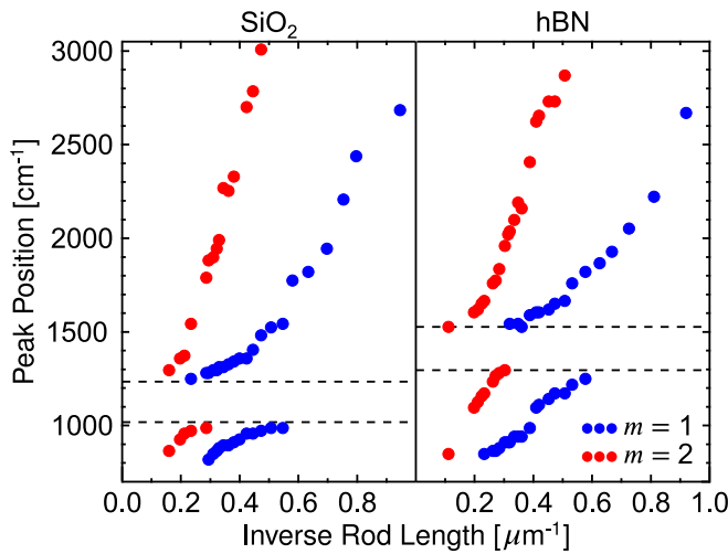
FIG. 4. Avoided crossing diagram derived from the SINS magnitude measurements for the complete nanorod series on both \text{SiO}_2 and hBN substrates. The m = 1 (blue) and m = 2 (red) FP modes are plotted versus inverse nanorod length. Dotted black lines are the asymptotic energies.
