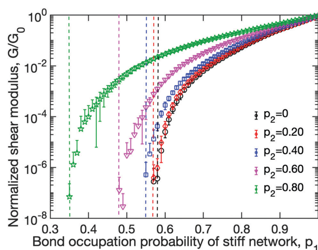
Fig. 2 The normalized shear modulus ( G/G_0 ) shown as a function of p_1 for an SN (black circles) and four DNs (remaining data). The values of p_2 are shown in the legend. The dashed lines guide to the eye for the rigidity percolation transitions. The data is averaged over five runs and the standard deviations are indicated by errorbars.
