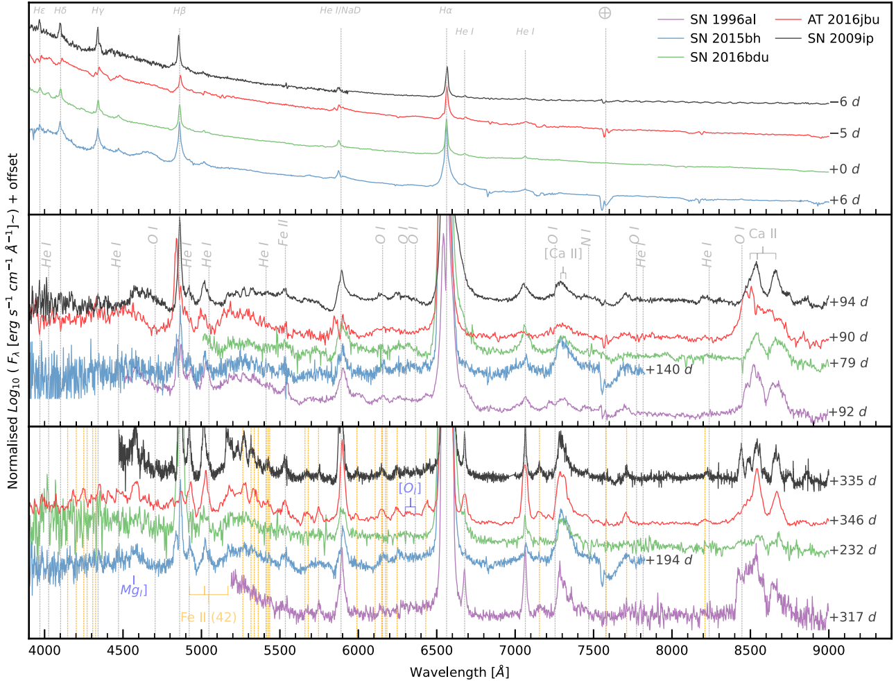
Figure 12. Spectral comparison of SN 2009ip-like transients around Event B peak (top), 3 months after Event B (middle), and late-time spectra around 1 yr later (bottom). We include several strong Fe II emission lines in the bottom panel as orange vertical lines. We note the remarkable similarities between AT 2016jbu and other SN 2009ip-like transients at late times.
