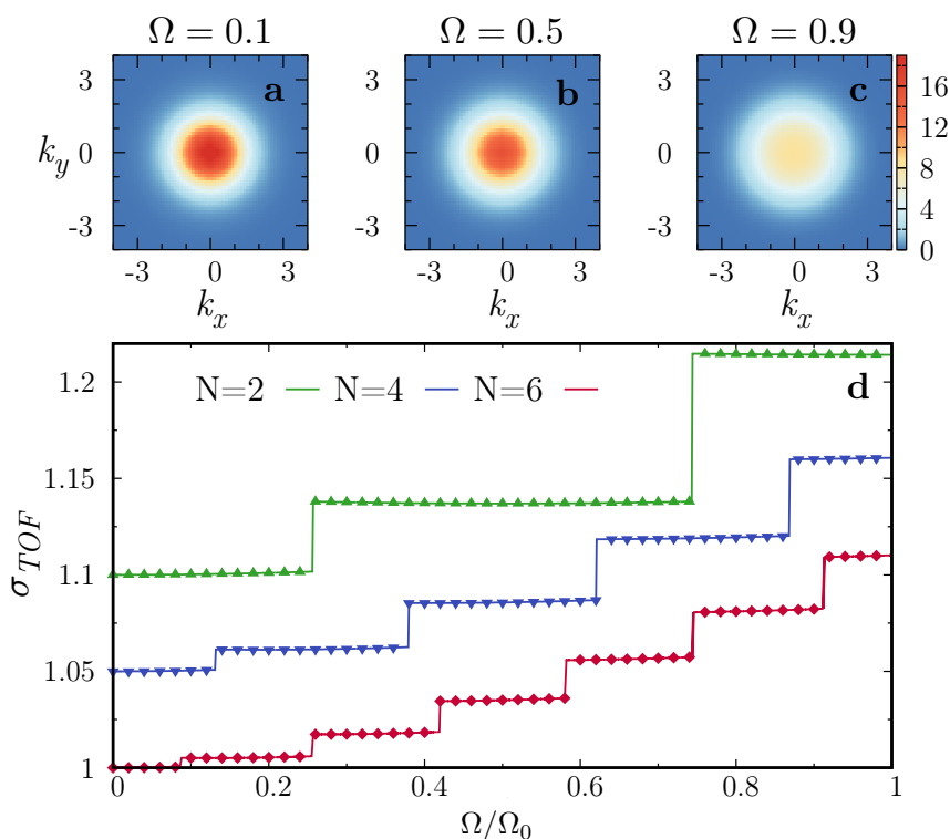
Figure 3: a-b-c Density plot of the TOF expansion for different values of the artificial gauge field in a system of N = 4 particles and N_s = 11 lattice sites. d Renormalized width \sigma_{\text{TOF}}/\sigma_{\text{TOF}}(\Omega = 0) of the time of flight density distribution, n(\mathbf{k}) . Green data are for N = 2 and U/J = -3 , blue for N = 4 and U/J = -1 and red for N = 6 and U/J = -0.6 . For the sake of graphical clarity, each curve is offset by 0.05. Note how the TOF density distribution width abruptly changes with the increase of the strength of the artificial gauge field, and how the sensitivity proportionally increases with the number of particles. In all the calculations we have approximated the Wannier functions with Gaussians functions with width \delta = a/\sqrt{2\pi} with a the lattice spacing.
