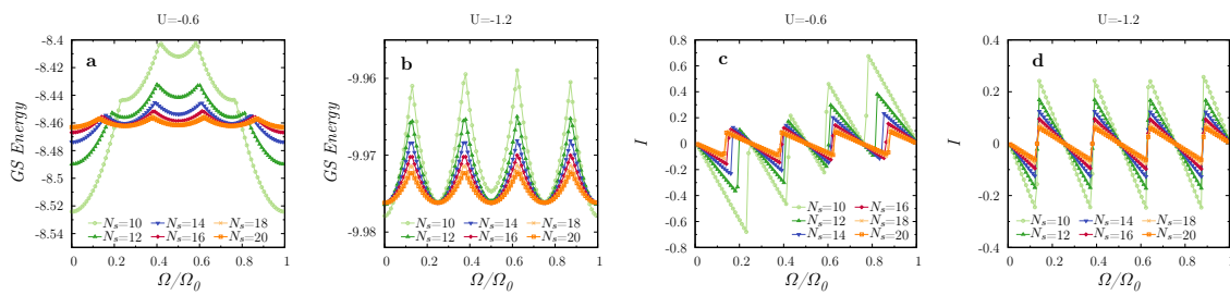
Figure 8: a, b ground state energy for different interaction as a function of the flux. c, d current, calculated as I = -\partial E_{GS}(\Omega)/\partial \Omega , for different interaction as a function of the flux.
