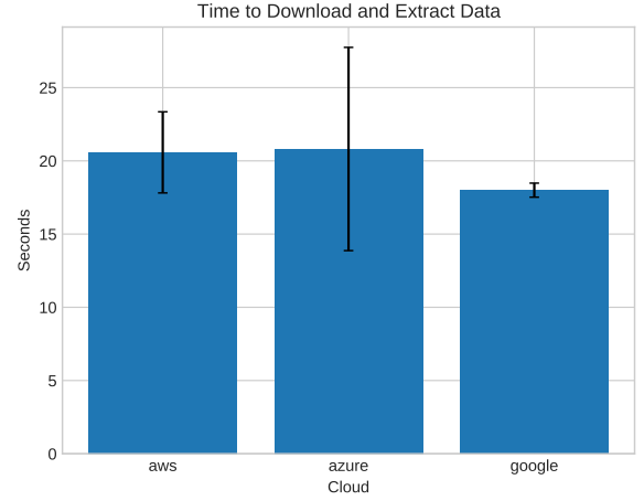
Fig. 12. Runtime for downloading the data used in the Eigenfaces SVM benchmark.
