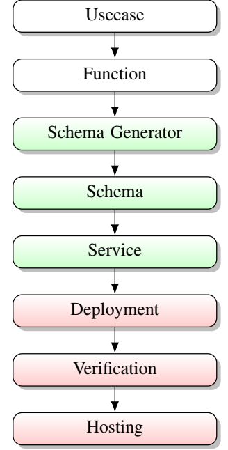
Fig. 5. Function-based component flow to specify an analytics service.
