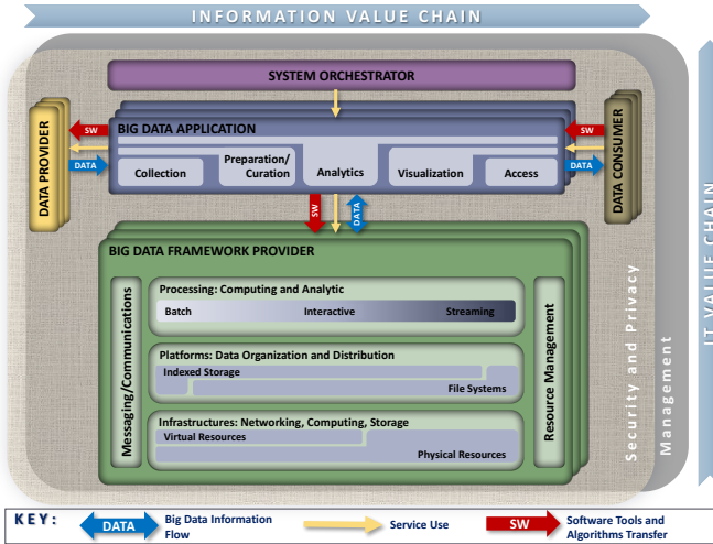
Fig. 1. NIST Big Data Reference Architecture [7]
