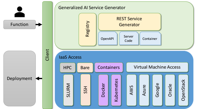
Fig. 3. Layered architecture of the cloudmesh OpenAPI framework.
