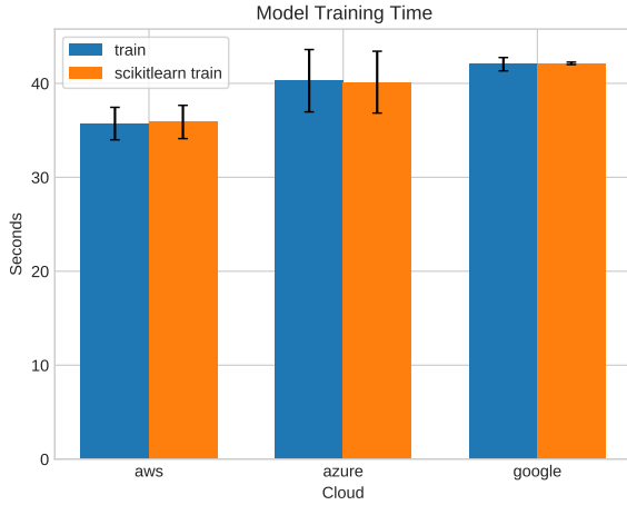
Fig. 14. Closeup of the Runtime for training on the data used in the Eigenfaces SVM benchmark without the data for the Pi.
