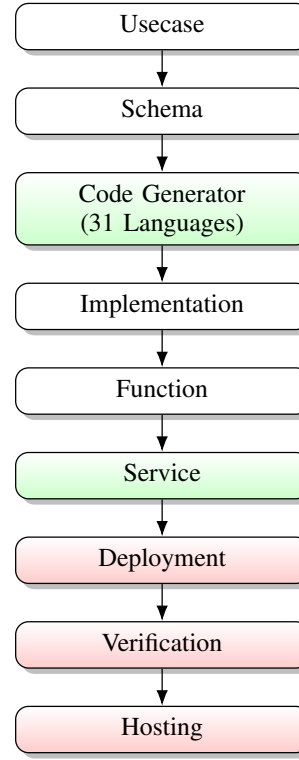
Fig. 4. Schema-based component flow to specify an analytics service.
