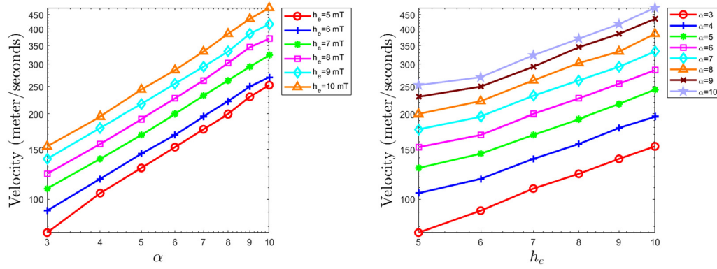
Fig. 6. Linear dependence of the wall velocity with respect to the damping parameter \alpha (left) and the external magnetic field h_e (right).
