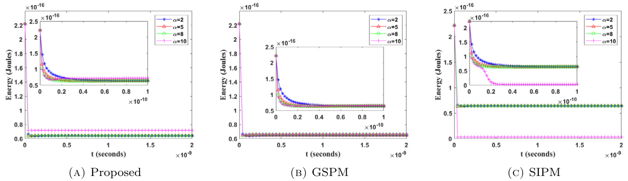
Fig. 3. Energy evolution curves of three numerical methods, with different damping constants, \alpha = 2, 5, 8, 10 , up to t = 2 ns in the absence of external magnetic field. Left: Proposed numerical method; Middle: GSPM; Right: SIPM. One common feature is that the energy dissipation rate is faster for larger \alpha , which is physically reasonable.
