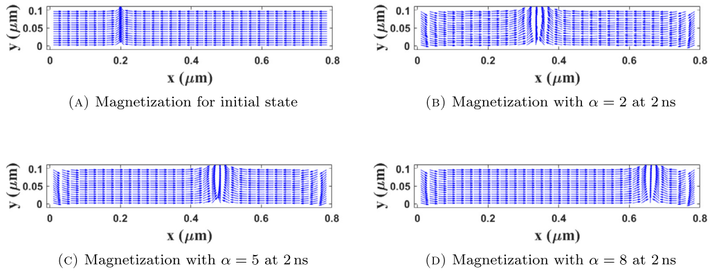
Fig. 5. Magnetization profiles of Neél wall motion in the presence of a magnetic field h_e = 5 mT, with \alpha = 2, 5, 8 at 2 ns for the proposed numerical method. The in-plane arrow denotes the first two components of the magnetization vector. The wall moves faster for larger values of \alpha and its velocity depends linearly on \alpha .
