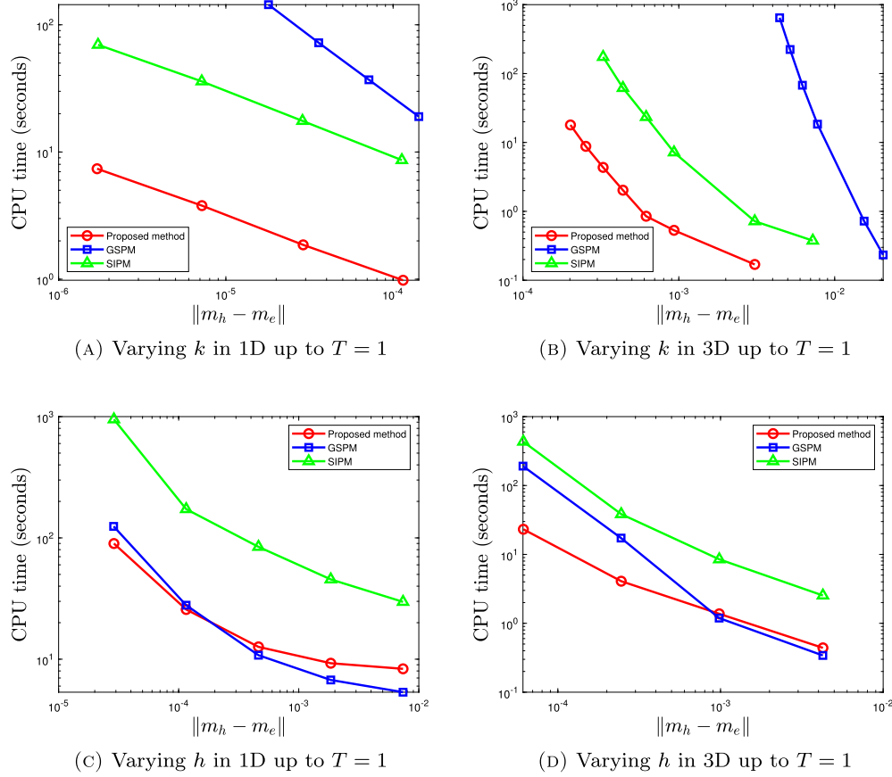
Fig. 1. CPU time needed to achieve the desired numerical accuracy, for the proposed method, the GSPM and the SIPM, in both the 1D and 3D computations. The CPU time is recorded as a function of the approximation error by varying k or h independently. CPU time with varying k : proposed method < SIPM < GSPM; CPU time with varying h : proposed method \approx GSPM < SIPM.
