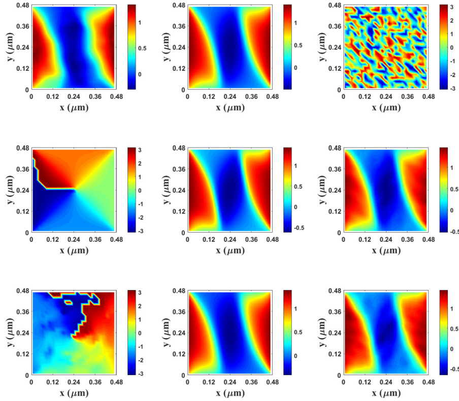
Fig. 2. Stable structures in the absence of magnetic field at 2 ns when \alpha = 0.01, 10, 40 . The color denotes the angle between the first two components of the magnetization vector. Top: Proposed method; Middle: GSPM; Bottom: SIPM. Left: \alpha = 40 ; Middle: \alpha = 10 ; Right: \alpha = 0.01 . (For interpretation of the colors in the figure(s), the reader is referred to the web version of this article.)
