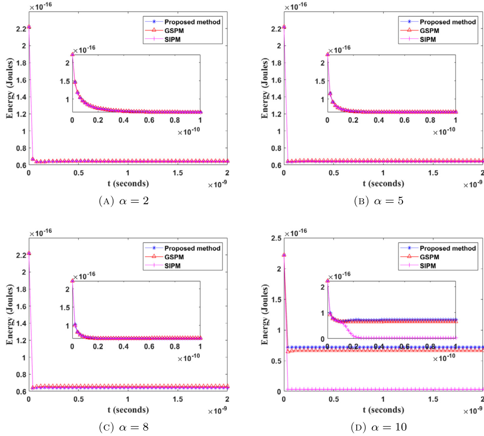
Fig. 4. Energy evolution curves in terms of time, for the numerical results created by three numerical methods up to t = 2 ns in the absence of external magnetic field for (a) \alpha = 2 , (b) \alpha = 5 , (c) \alpha = 8 , and (d) \alpha = 10 . The energy dissipation pattern of the proposed method is consistent with the other two methods for (a), (b), and (c), and the SIPM has a slightly different energy dissipation pattern from the other two methods for (d).
