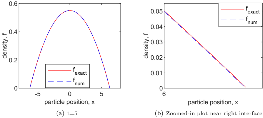
FIG. 8.3. The density f at time t=5 and zoomed-in plot near right interface with the exact solution f_{\text{exact}} and the numerical solution f_{\text{num}} ( M=100 , \Delta t=1/100 ).
