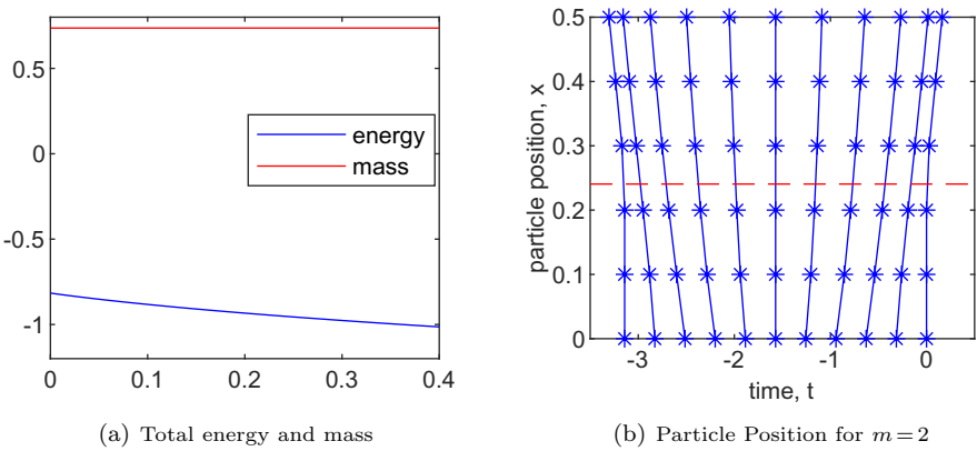
FIG. 8.6. The evolution of total energy, total mass and particle position ( M=100 , \Delta t=1/2000 ).
