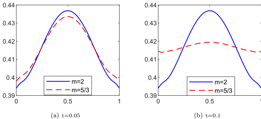
FIG. 8.1. The density f at time t=0.05 and t=0.1 ( h=1/100 , \Delta t=1/100 ).
