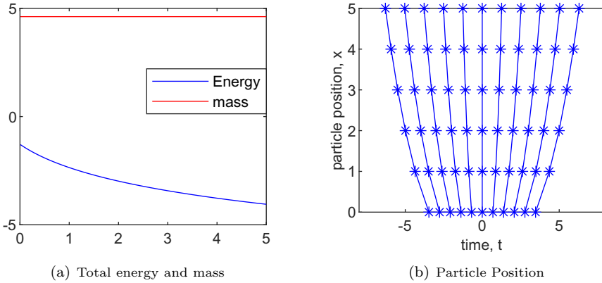
FIG. 8.4. The evolution of total energy, total mass and particle position for m=2 ( M=100 , \Delta t=1/100 ).
