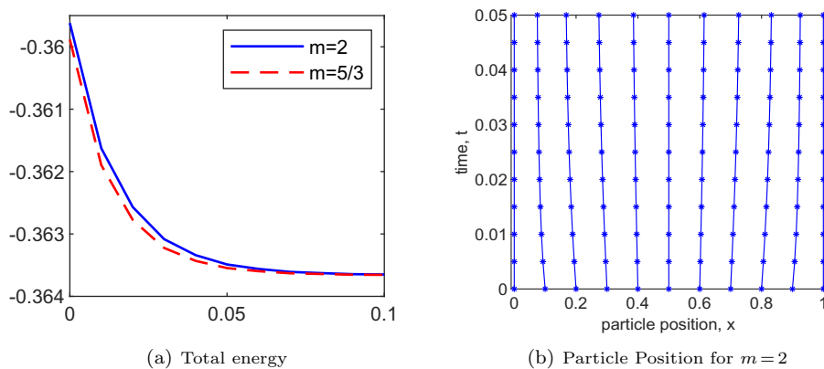
FIG. 8.2. The evolution of total energy and particle position ( h=1/100 , \Delta t=1/100 ).
