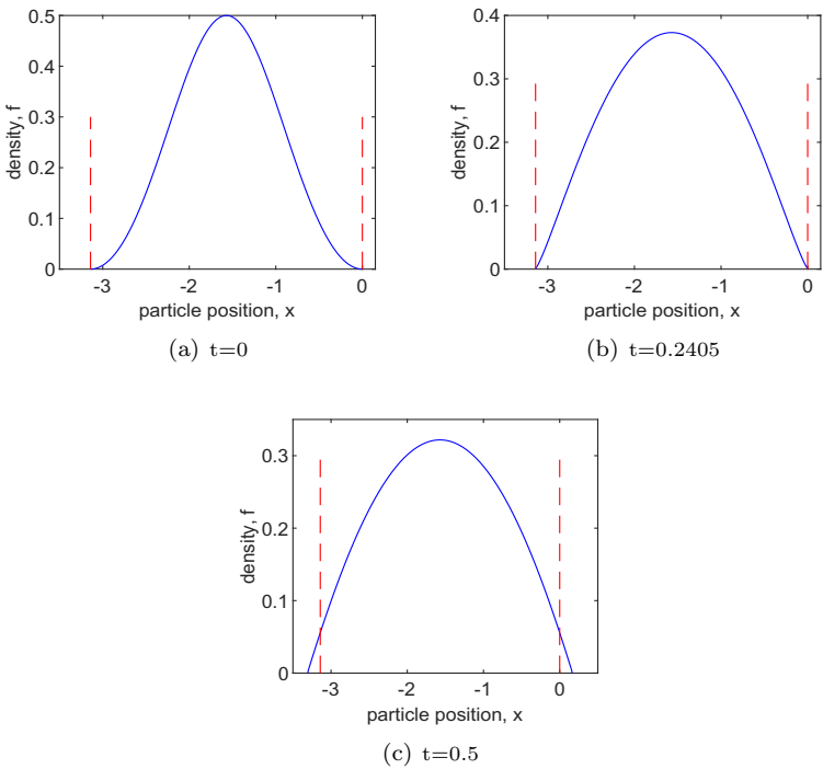
FIG. 8.5. The evolution of density f with m=2 ( M=100 , \Delta t=1/2000 ).
