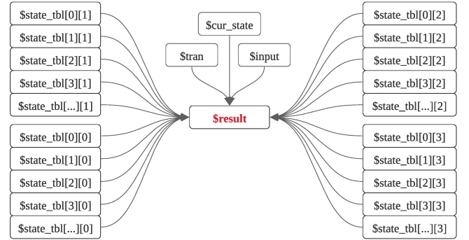
Figure 7: Data Dependency Graph by Taint Analysis.
