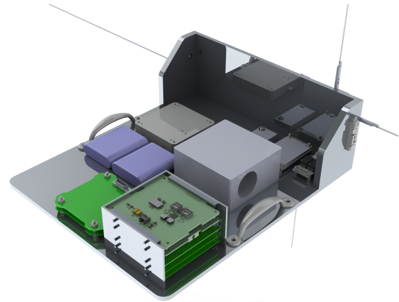
Figure 7: Rendering of assembled SWARM-EX FlatSat as of May 2021.
