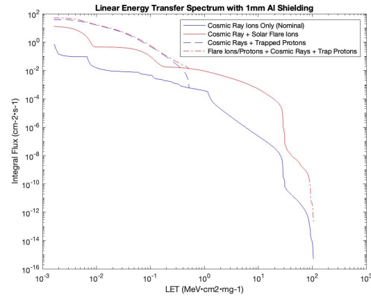
Figure 2: Integral LET spectrum for a 500 km orbit through 1 mm of Al shielding. The various curves show the levels of transported particle flux through a specified shielding for various sets of environment particles.
