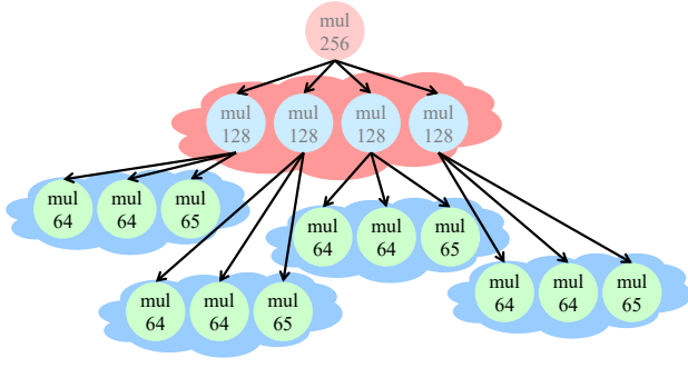
Fig. 1: Schoolbook followed by Karatsuba decomposition of 256-bit integer multiplication. Each node is a partial product implemented using DSPs and LUTs. Cloud shapes represent the summation of the partial products and are implemented using LUTs.
