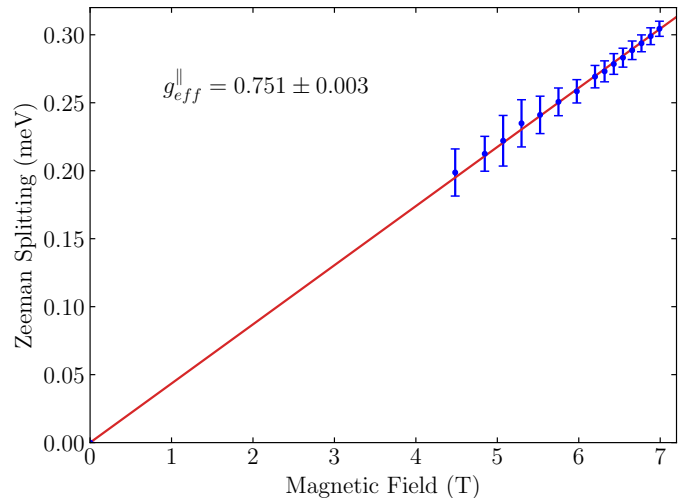
FIG. 11. Zeeman splitting of the Ga donor lines as a function of magnetic field at 5.2 K in the Faraday geometry. Each point is obtained via Voigt profile fits on PL spectra under 3.45 eV excitation at different fields. The error bars depict the standard deviation error of the Voigt profile fits.
