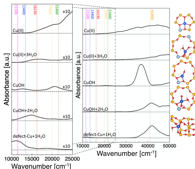
Figure 3: Theoretically predicted optical spectra for different Cu monomers in Cu-SSZ-13 between 10000 cm -1 and 25000 cm -1 (left panel) and between 10000 cm -1 and 50000 cm -1 (right). Spectra are shown as solid black lines and the zero-intensity line for each spectrum is shown as a horizontal dashed black line. Experimentally observed peaks and shoulders are marked with dashed, vertical lines in various colors for readability. For better visibility, spectra in the left panel have been multiplied by the factor indicated by each spectrum. Colors in atomistic pictures on the right correspond to Figure 1.
