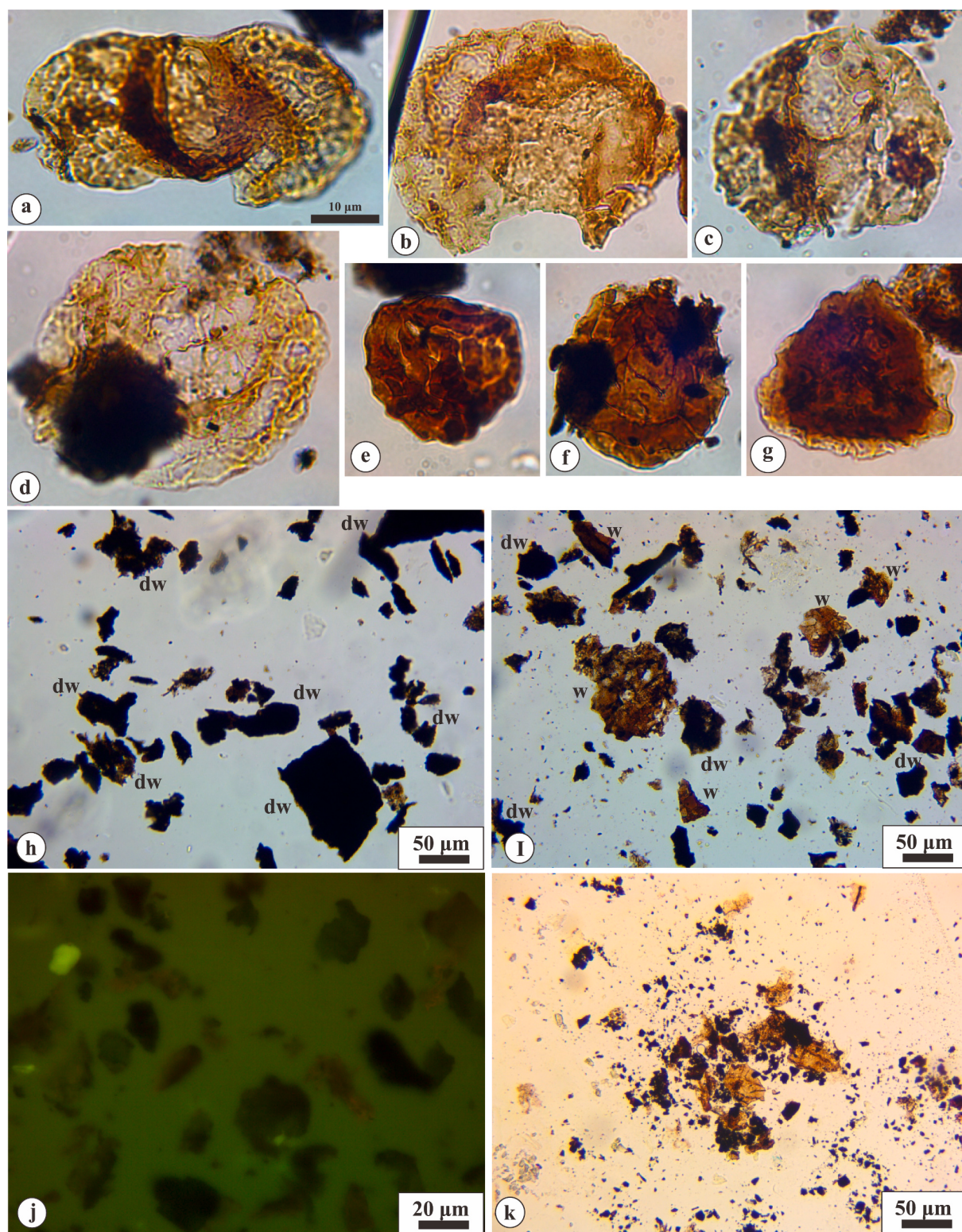
Fig. 5. Selected palynomorphs (a-g) and palynofacies (h-k) from the core Z40. Scale bar of 10 μm shown as bar (a) applies to each palynomorph image in (a-g). (a) Platysaccus queenslandi , 1380.6 m level. (b) Florinites? sp. 1361.1 m. (c) Chordasporites sp. 1455 m. (d) Parataeniaesporites striatus 1410.2 m. (e-f) Asseretospora sp. 1380.6 m. (g) Kreuselispores guangyuensis 1374.6 m. (h) Palynofacies at 1474.4 m with a predominance of degraded "pseudoamorphous" black-brown wood particles (dw). (i) Palynofacies at 1420.3 m with predominantly degraded "pseudomorphs" wood (dw) and biostructured phytoclasts (w). Despite the lack of distinct structure and "fuzzy" edges, the angular-tabular appearance of these particles indicate a terrestrial origin. (j) Palynofacies at 1420.3 m in fluorescence light. Note the total lack or very weak fluorescence of the organic particles. (k) Palynofacies at 1361.1 m. Note the increase of more transparent plant debris, but the degraded particles with pseudoamorphous appearance are still predominant. (For interpretation of the references to colour in this figure legend, the reader is referred to the web version of this article.)
