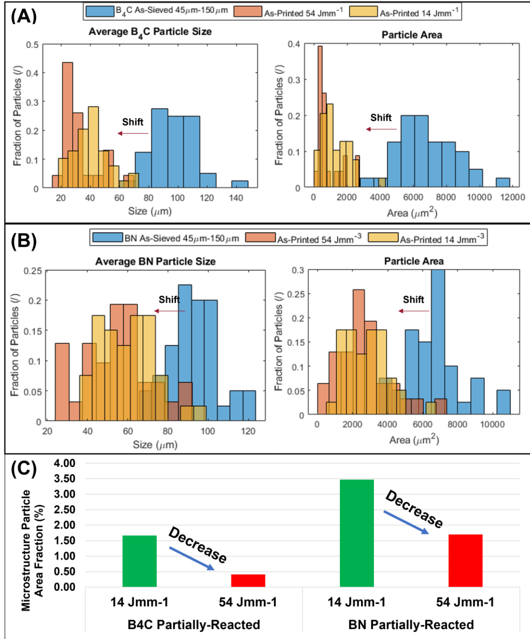
Figure 6: PSD distribution of B 4 C and BN particles at different processing conditions in comparison to as-sieved condition. Note: 20-40 measured particles contribute to each distribution. (A) B 4 C. (B) BN. (C) Comparison of overall area fraction of as-processed particle sizes in the microstructure for each reinforcement and processing parameter set.
