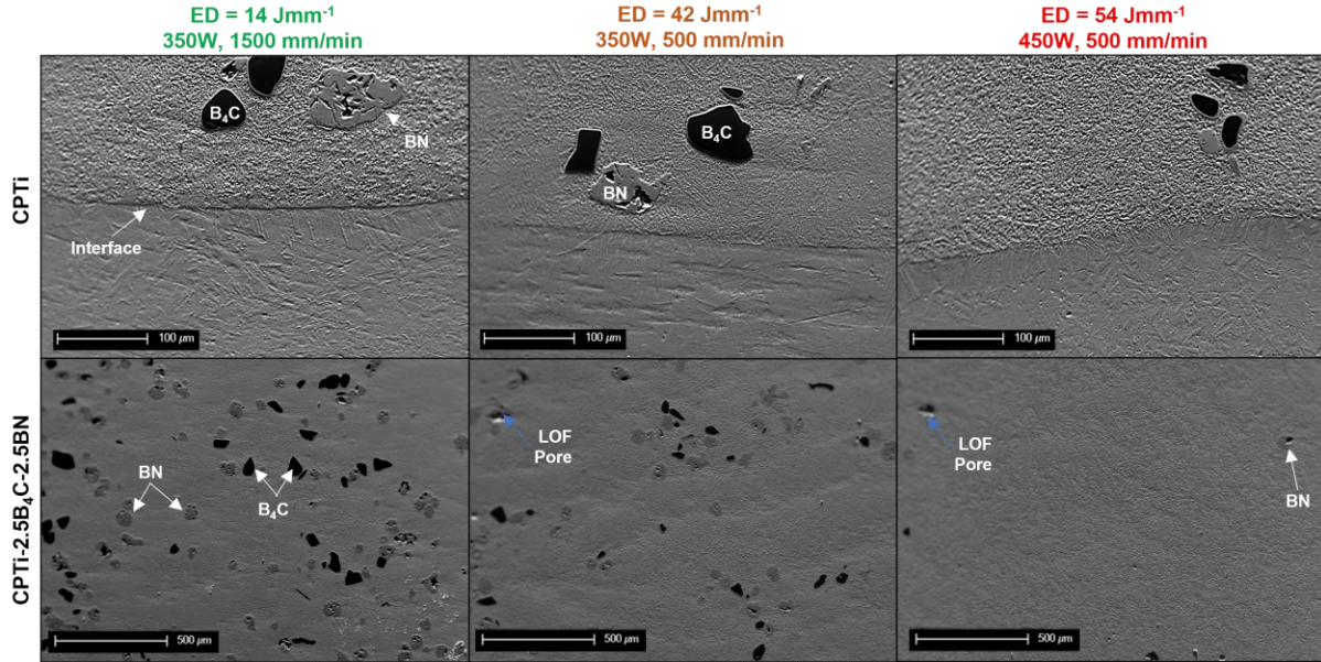
Figure 3: Comparison of interfaces and low-magnification images of bulk samples processed at 14-54 \text{Jmm}^{-1} input energy density. ( Top Row ) CPTi, and ( Bottom Row ) CPTi-2.5B 4 C-BN.
