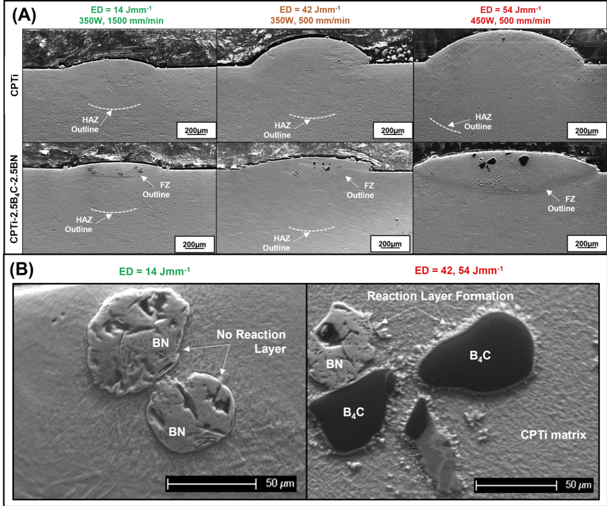
Figure 2: Comparison of low and high-magnification images of tracks at 14-54 Jmm -1 input energy density. (A) Single tracks of both CPTi and CPTi-B 4 C-BN, and (B) Comparison of CPTi-B 4 C-BN processed at both low and high input energy density.
