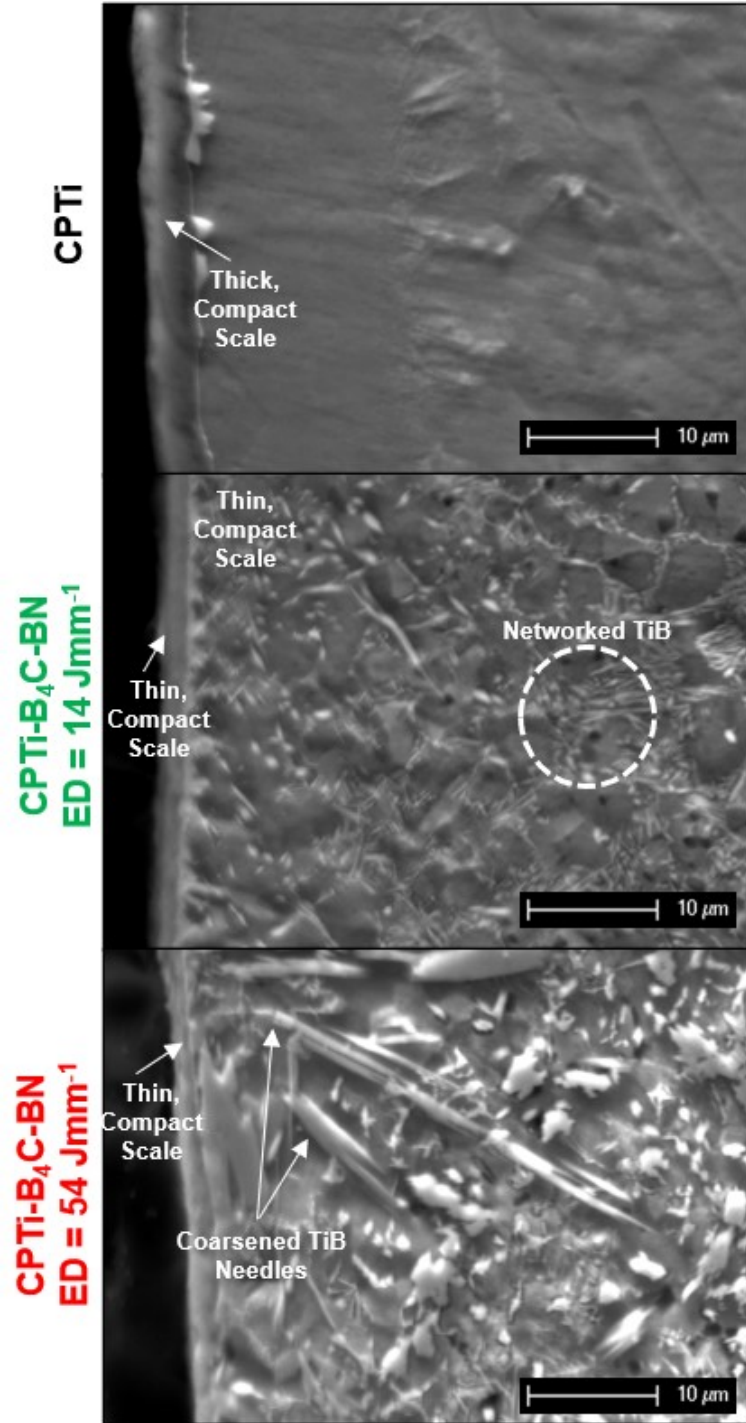
Figure 10: Comparison of oxide scale cross sections of both the CPTi and CPTi-B 4 C-BN compositions at different input energies.
