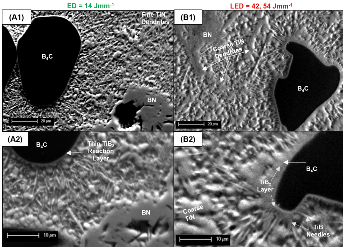
Figure 4: High magnification microstructures of variable process parameter samples. (A1 & A2) 14 \text{Jmm}^{-1} at increasing magnification, and (B1 & B2) 42-54 \text{Jmm}^{-1} at increasing magnification.
