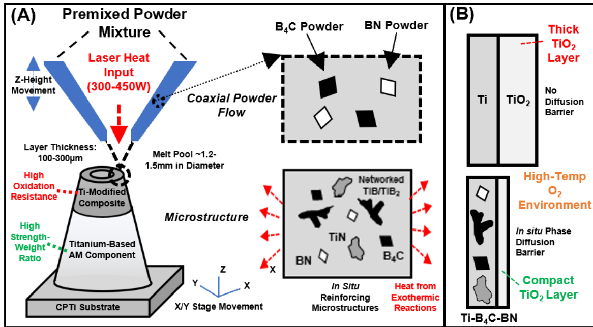
Figure 1: Reactive-based reinforcement concept for titanium-based components. (A) Processing via directed energy deposition technology (DED). (B) Performance improvement using ceramic reinforcement for increased oxidation resistance.
