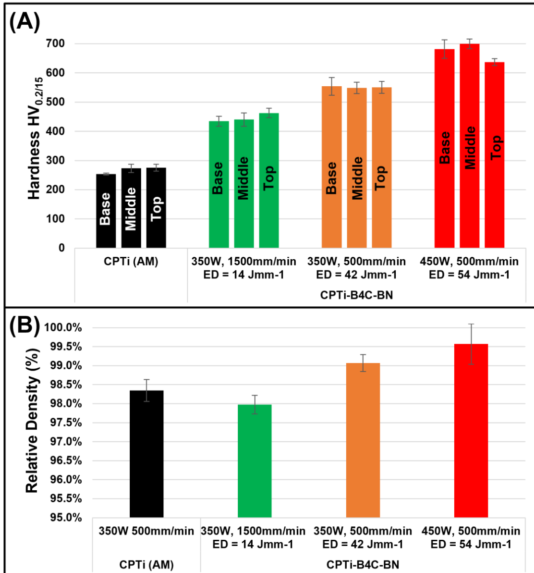
Figure 7: Hardness and relative density of composites at different processing conditions. (A) Hardness of each energy density within the base, middle, and top of the deposits. (B) Relative density of each energy density in comparison to CPTi. Note that relative density was calculated with respect to the theoretical composite composition.
