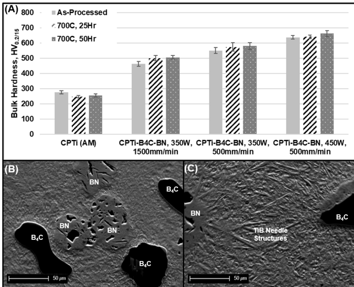
Figure 11: Hardness and microstructures of as-oxidized specimens. (A) Hardness of each composition and process parameter set after both 25hr and 50hr tests at 700°C. (B) Microstructure of CPTi-B 4 C-BN composition processed at 14 \text{ Jmm}^{-1} . (C) Microstructure of CPTi-B 4 C-BN composition processed at 54 \text{ Jmm}^{-1} .
