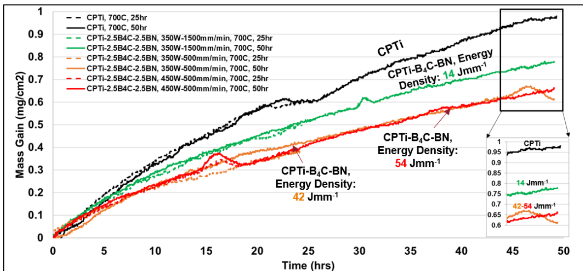
Figure 8: Thermogravimetric curves of each composition and processing parameters for both 25hrs. and 50hrs at 700°C in air. Note: dashed curves represent the 25hr runs.
