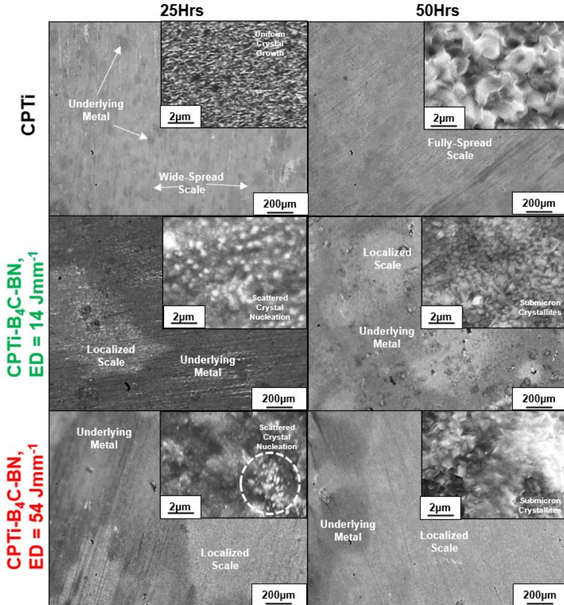
Figure 9: Comparison of oxide scales on surface of both CPTi and CPTi-B 4 C-BN compositions at different input energies and at each time point. Inset images are the same sample at high magnification.
