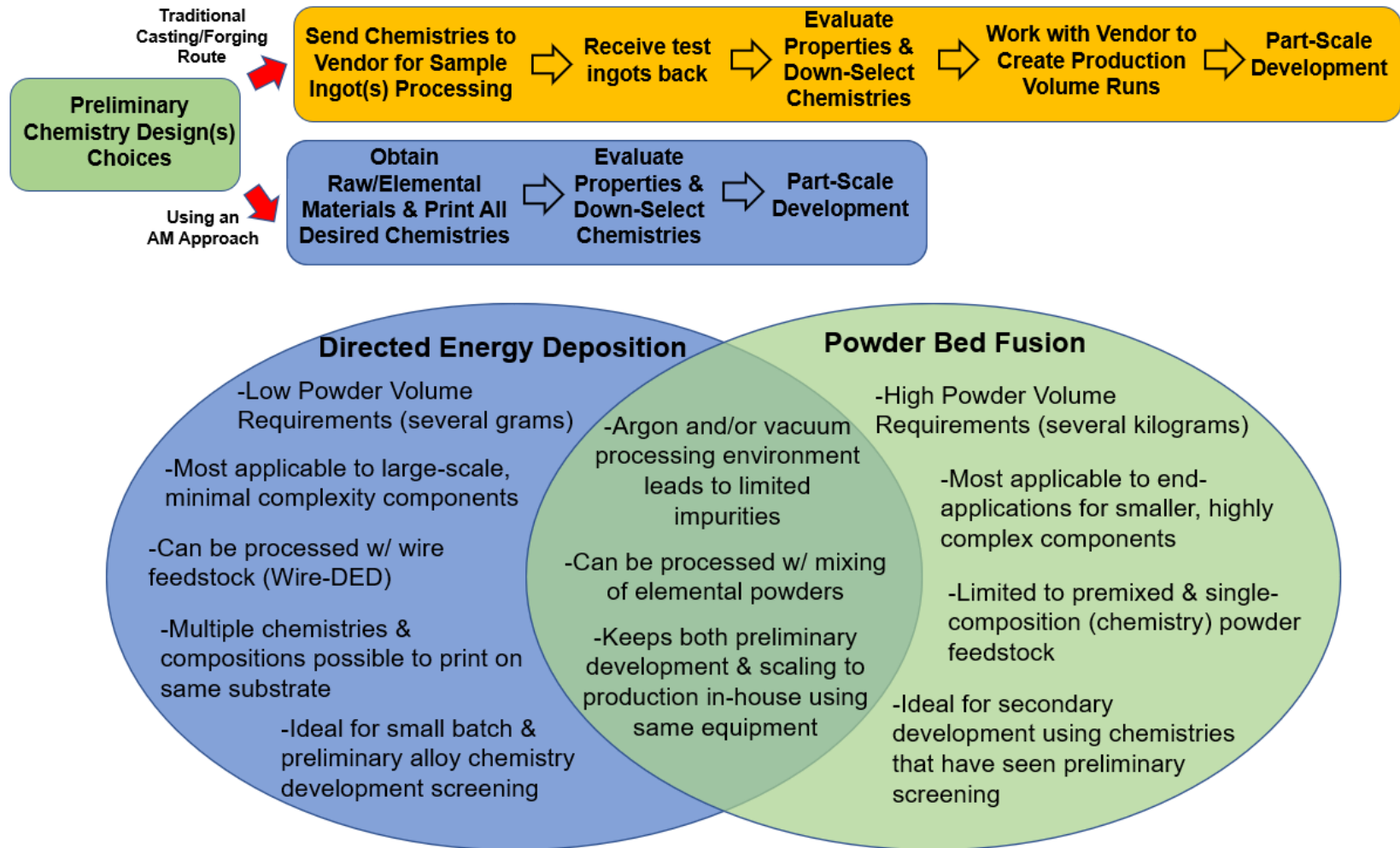
FIGURE 2. Comparison of alloy design approaches using traditional methods and the main metal-based AM methods –directed energy deposition (DED) and powder bed fusion (PBF).
