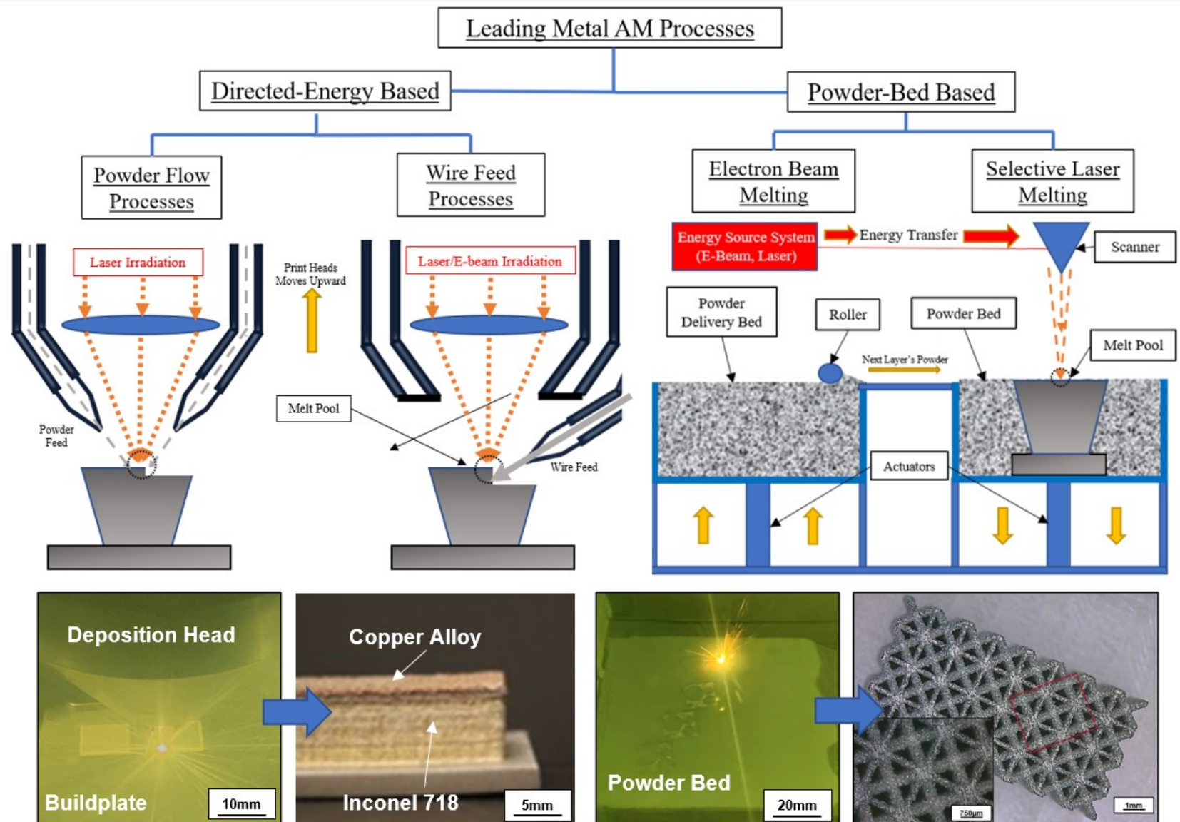
FIGURE 3. Directed energy deposition (DED) and Powder bed fusion (PBF) based additive manufacturing methods [24,6].
