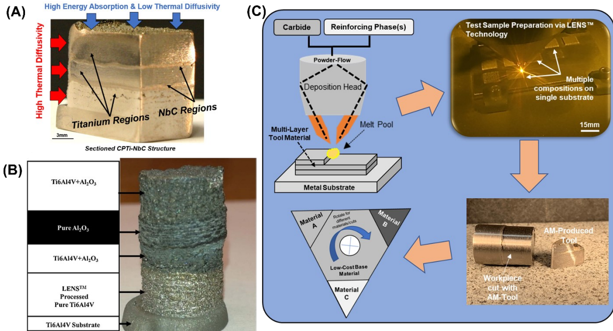
FIGURE 10. Examples of metal-ceramic composite material development. (A) Layered metal-ceramic composite [84]. (B) Titanium to alumina structure [101]. (C) Diamond reinforced cutting tool design using DED [85].
