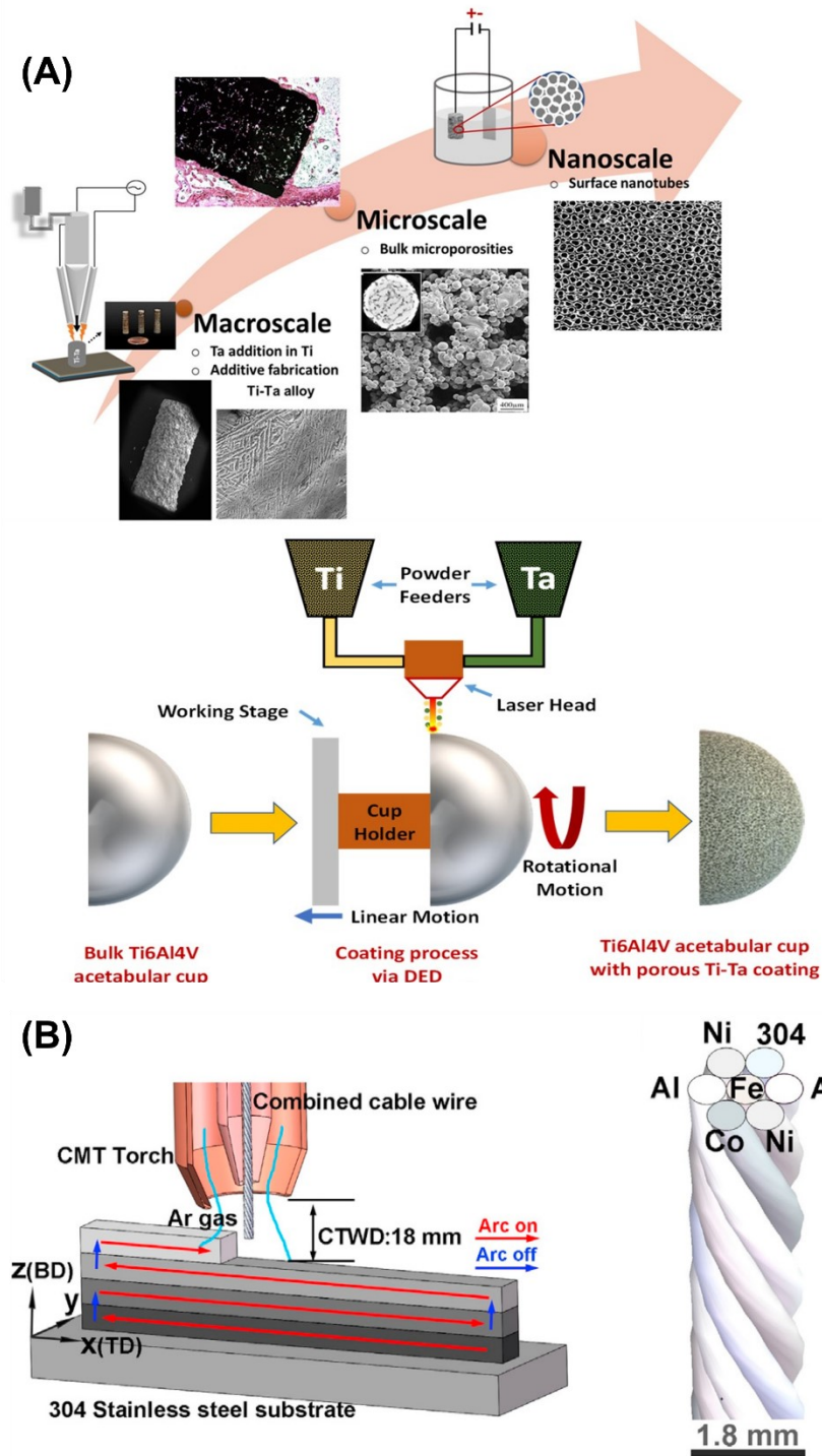
FIGURE 8. Novel multi-material concepts in alloy design using AM. (A) Application of DED to design Ti-Ta alloys to increase biocompatibility and balance processability challenges of incorporating tantalum in the microstructure [27]. (B) Combined cable concept for multi-material AM using wire-based DED [77].
