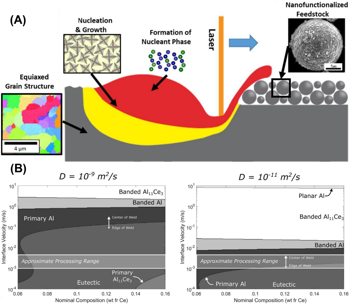
FIGURE 6. Examples of alloy design are being utilized in the development of aluminum-based materials. (A) Schematic showing the influence of the inoculant phase on the resulting equiaxed microstructure after solidification [64]. (B) Resulting microstructures projected via computation coupled with experiments in the development of Al-Ce class of alloys [56].
