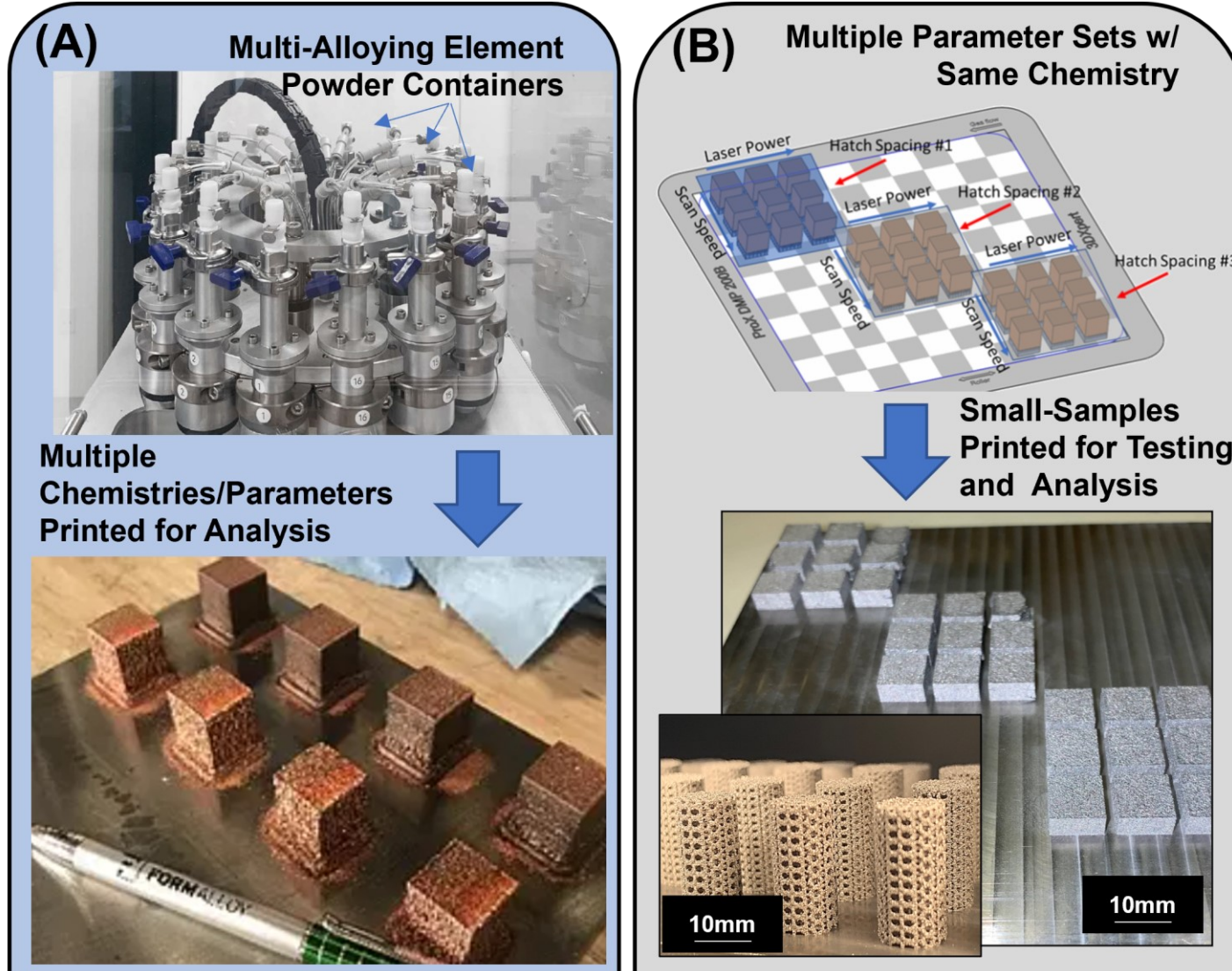
FIGURE 4. Examples of alloy design projects using both (A) the DED [14], and (B) the PBF.
