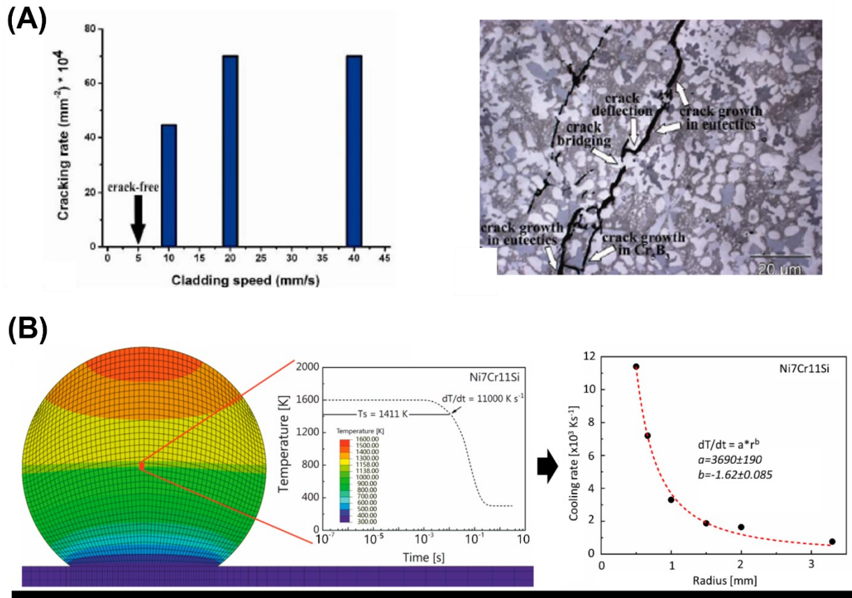
FIGURE 5. Examples of alloy design characteristics of Fe- and Ni-based alloys in the literature. (A) Example of scanning speed effects on microcracking in Cr-Si-B modified Ni-based alloy [50]. (B) Example of a droplet-based simulation to understand the effects of cooling rate on the resulting microstructures of Ni-Cr-Si ternary system during laser-based AM [51].
