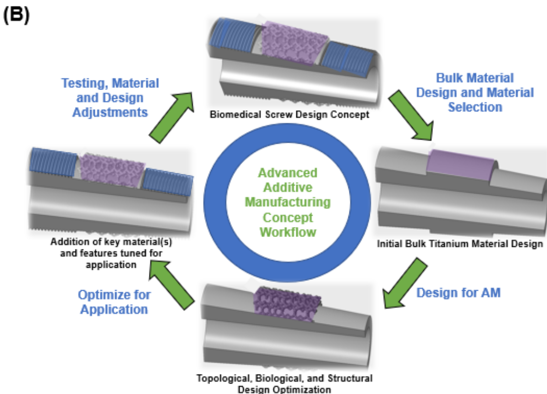
FIGURE 1. Example of current alloy design approach using laser-based additive manufacturing.
