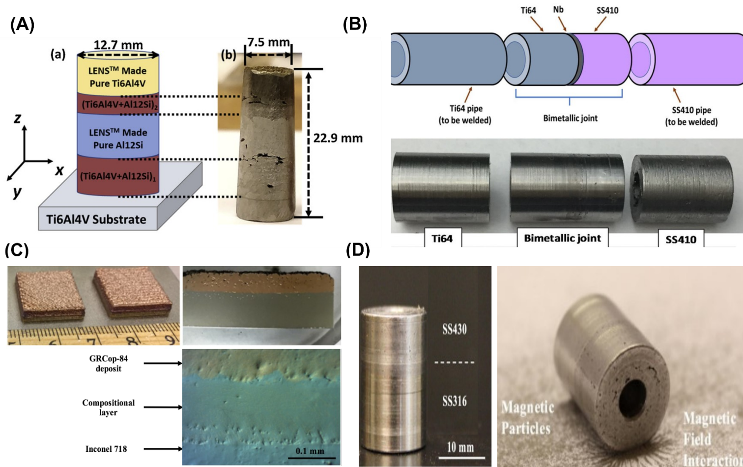
FIGURE 9. Examples of next-generation functionally-graded materials (FGMs) and related efforts towards achieving such structures with variable processing strategies. (A) Processing of Ti–6Al–4V/Al12Si joints [28]. (B) Bimetallic structures fabricated from Ti–6Al–4V and SS410 [30]. Increased diffusivity from deposition of copper alloy on Inconel 718 [31]. Magnetic-non magnetic joints are made from different stainless steel [102].
