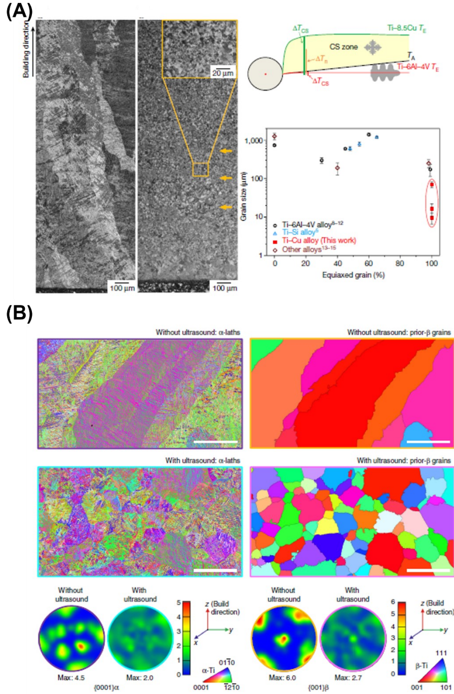
FIGURE 7. Examples of titanium-based alloy development via AM. (A) Copper-modified titanium influence a columnar to equiaxed grain structure [57]. (B) Effect of ultrasonic vibrations on grain refinement and reduction of columnar structures in DED-based processing of titanium alloys showing absence of texture and equiaxed microstructure [70].
