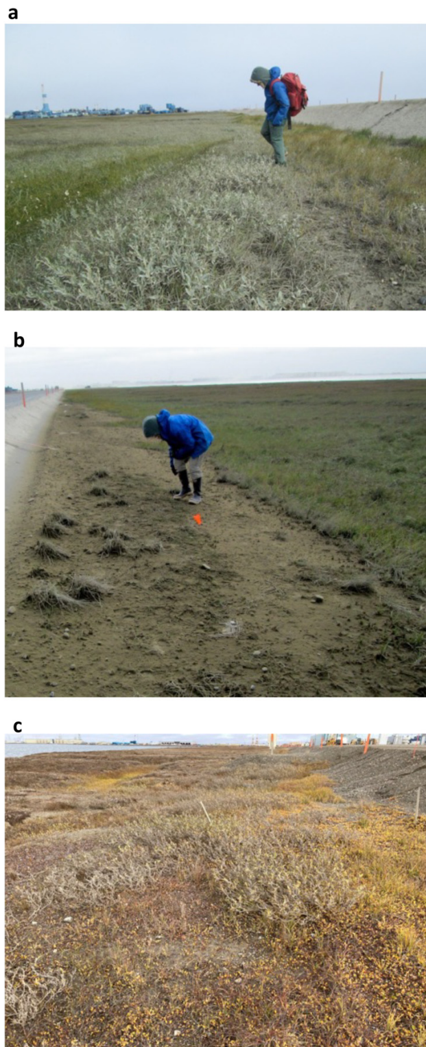
Fig. 15. (a) Strip of 25-cm tall erect dwarf willows ( Salix richardsonii ) growing on NE (T1) side of the road along the line of a buried utility trench. The area at the base of the road embankment has high concentration of grasses. (b) Heavily dusted roadside area on the SW (leeward) side of the road. Numerous salt-tolerant species such as Puccinellia andersonii and Puccinellia phryganodes occur on the barren slope that has been created by the heavy dust. (c) Roadside willows ( Salix richardsonii ) up to 1 m tall growing near the Deadhorse Airport and the south side of Lake Colleen.
