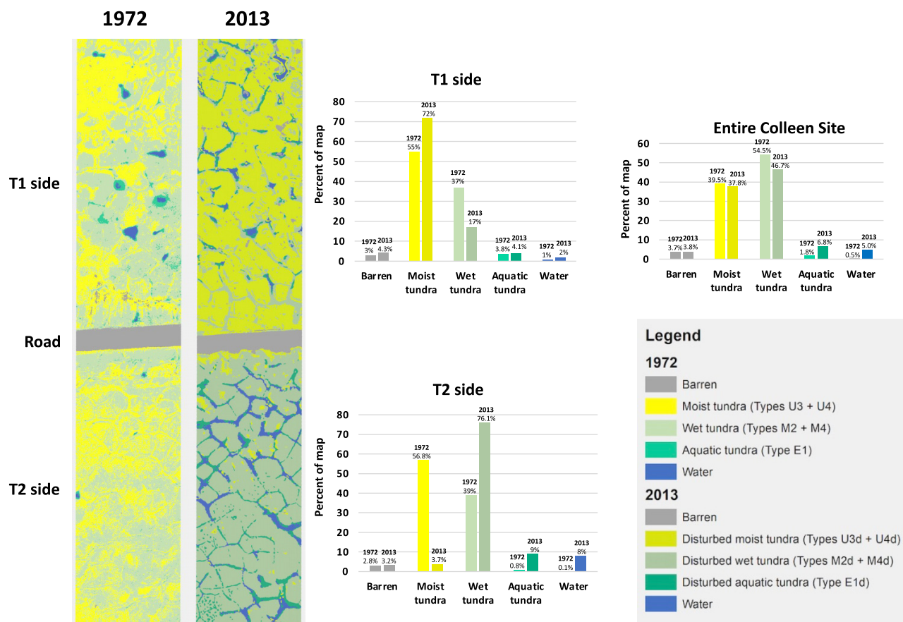
Fig. 12. Vegetation maps and analysis of the Colleen site in 1972 and 2013. The road was constructed in 1969 when the vegetation patterns were still like those prior to road construction. The maps illustrate the damming effect of the road, which prevents drainage of water from the T2 (SW) side of the road to the T1 (NE) side. Bar graphs show the distribution of broad vegetation types and water. (Derived from Raynolds et al. 2014b ).
