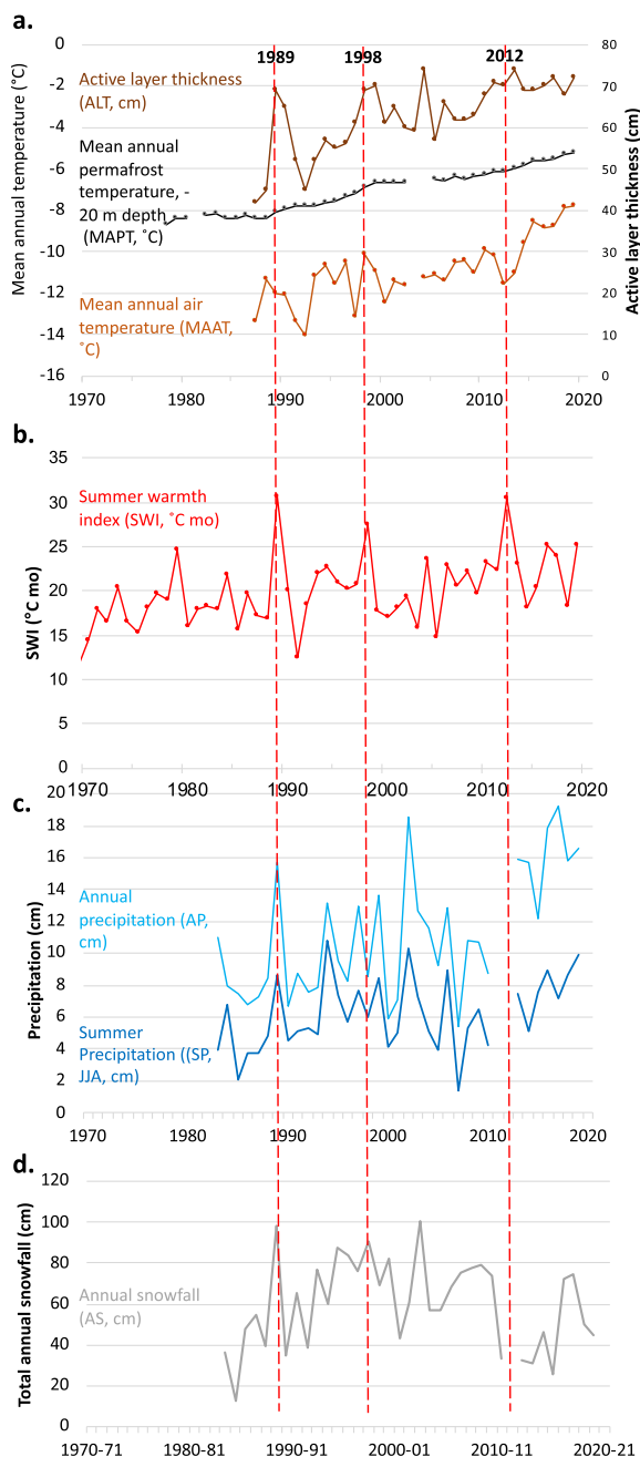
Fig. 5. Prudhoe Bay climate and thaw-depth trends: (a) Brown line: Active layer thickness (ALT, 1988–2019). Black line: mean annual permafrost temperature (MAPT, 1978–2019). Orange line: mean annual air temperature (MAAT, 1986–2019). Data are from Romanovsky's Deadhorse site ( https://permafrost.gi.alaska.edu/site/dh1 ) (b) Red line: Summer warmth index (SWI = Annual sum of the monthly mean temperatures above freezing). The SWI graph combines two records from the Prudhoe (ARCO) Station (1969–1985; Thoman 1995 ) and the Deadhorse NWS Station (1986–2019, Western Regional Climate Center) (see Fig. 2 for locations). c. Precipitation (1983–2019). Light blue line: Annual precipitation; Dark blue line: Summer (JJA) precipitation (1983–2019). (d) Gray line: Annual snowfall (1982–1983 to 2019–2020). Data for c and d are from the Kuparuk Station (WRCC Station ID 505136). Red dashed vertical lines: Warm summers in 1989, 1998, and 2012.
