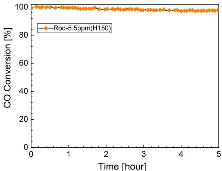
Figure S15. CO oxidation activity as a function of time at a temperature of 213 °C obtained over Rod-5.5ppm. Reaction conditions: CO=1.0 sccm, O 2 =10 sccm, Ar=10 sccm, He=79 sccm.
