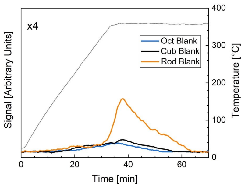
Figure S6. Temperature programmed reduction profiles collected from the bare rods, cubes and octahedra. Data is plotted on the same scale to facilitate comparison. However, the x4 on the y-axis indicates that the signal intensity of this figure was multiplied by four compared with Figure S5. The corresponding temperature ramping file is shown in gray..
