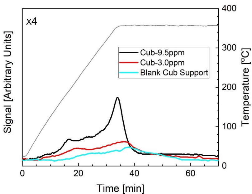
Figure S4. Temperature programmed reduction profiles collected from Cub-9.5ppm, Cub-3.0ppm and blank cube support. The corresponding temperature ramping file is shown in gray. The x4 on the y-axis indicates that the signal intensity of this figure was multiplied by four compared with Figure S5 to allow comparisons, while at the same time reveal detailed features in the TPR profiles of these catalysts with lower intensities.
