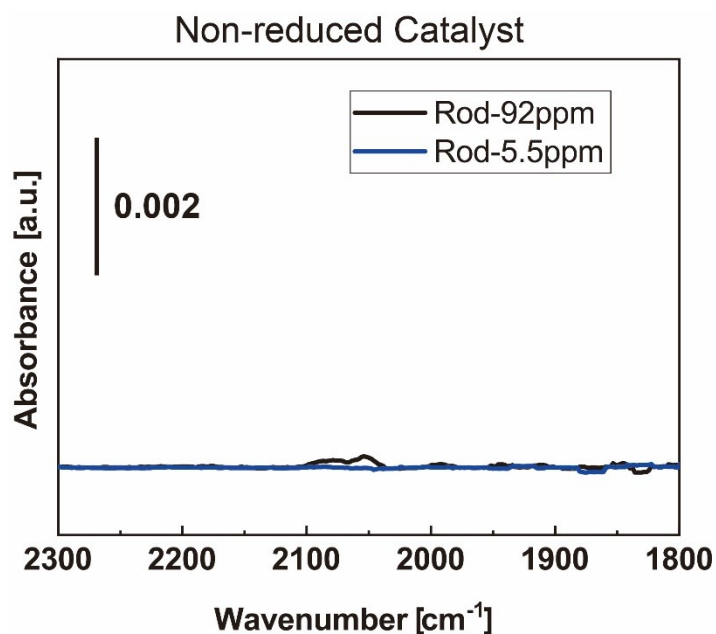
Figure S10. CO DRIFTS data collected from fresh (non-reduced) Rod-92ppm and Rod-5.5ppm catalysts after CO exposure at room temperature. The fresh catalysts were calcined at 350 °C for 3 hours under static air and degassed at 200 °C for 20 min in situ under 20 sccm He flow prior to the CO exposure.
