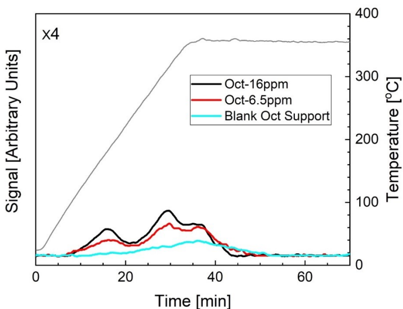
Figure S3. TPR profiles collected from Oct-16ppm, Oct-6.5ppm and blank octahedral support. The temperature measured as a function of time is shown in gray and displayed on the right y-axis. The x4 on the y-axis indicates that the signal intensity of this figure was multiplied by four compared with Figure S5 to allow comparisons, while at the same time reveal detailed features in the TPR profiles of these catalysts with lower intensities.
