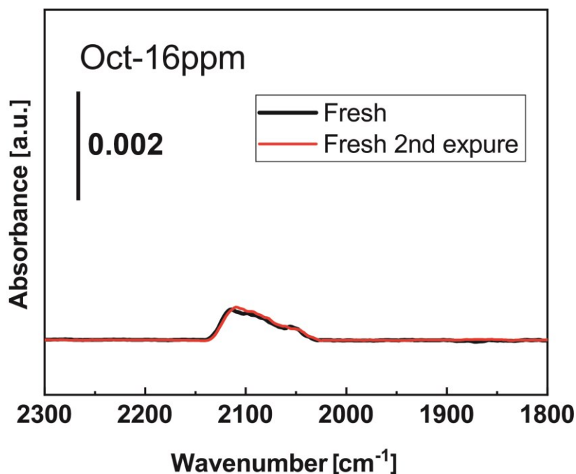
Figure S8. CO DRIFTS data collected from fresh (non-reduced) Oct-16ppm during two consecutive CO exposure at room temperature. Each CO exposure lasted 20 min under 20 sccm 5% CO balanced with N 2 . The fresh sample was calcined at 350 °C for 3 hours and was degassed at 200 °C for 20 min under 20 sccm He flow prior collecting the spectra.
