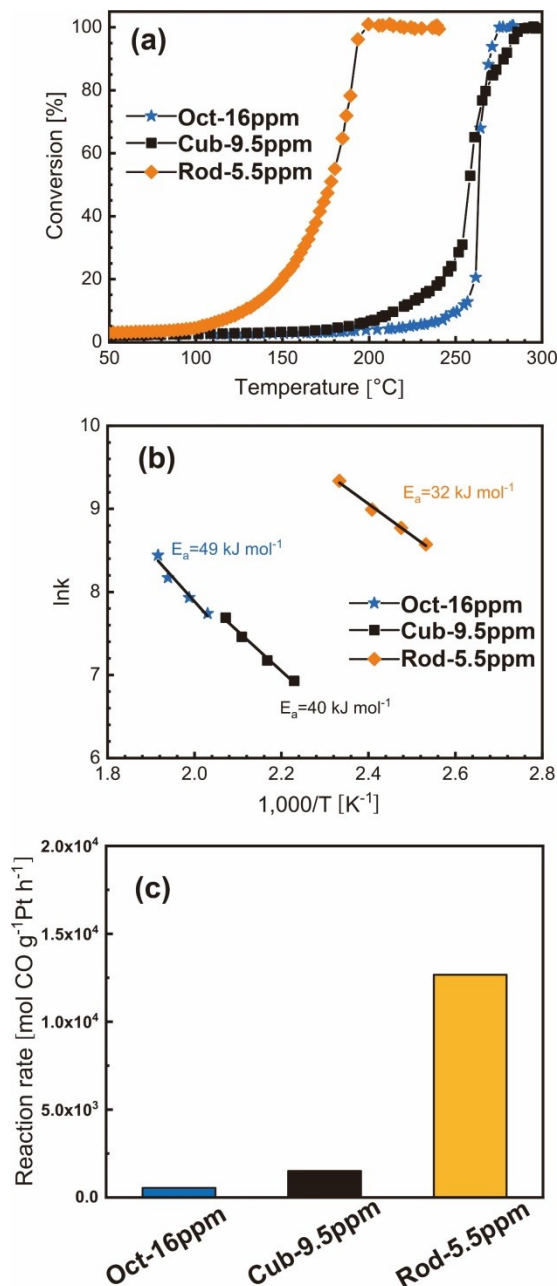
Figure 6 (a) The CO oxidation activity as a function of temperature over Oct-16ppm, Rod-5.5ppm, and Cub-9.5ppm. CO:O 2 :Ar:He = 1:10:10:79 sccm and heating rate 10 °C/min. (b) Arrhenius plot of CO oxidation rate with calculated activation energies for the same catalysts as in (a). (c) Reaction rate in mol CO converted per gram of Pt per hour at a temperature of 190 °C.
