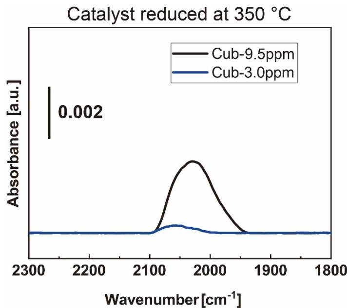
Figure S9. CO DRIFTS data collected from Cub-9.5ppm and Cub-3.0ppm. The samples were from the 350 °C TPR experiment and was mildly reduced at 200 °C for 20 min prior collecting the spectra (as described in the figure caption of Figure S7).
