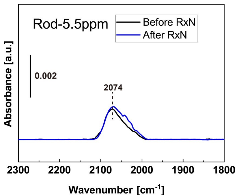
Figure S16. CO-DRIFTS data collected from Rod-5.5ppm after an in-situ exposure to CO oxidation conditions (CO=0.5 sccm, O 2 =5.0 sccm, He=44.5 sccm) at 213 °C inside the DRIFTS cell for 1 hour. After CO reaction, the catalyst was outgassed at 200 °C and cooled down in inert before being reduced at 150 °C (same procedure as for the fresh catalyst). The CO-DRIFTS spectra obtained from the Rod-5.5ppm catalyst after reaction are identical to those before reaction treatment, indicating the isolated Pt atoms were maintained on the surface.
