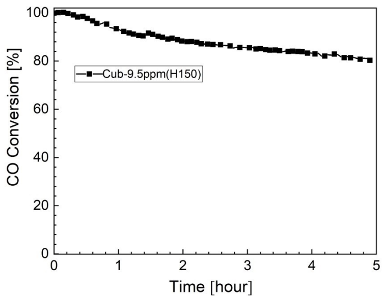
Figure S14. CO oxidation activity as a function of time at a temperature of 295 °C obtained over Cub-9.5ppm, Reaction conditions: CO=1.0 sccm, O 2 =10 sccm, Ar=10 sccm, He=79 sccm.
