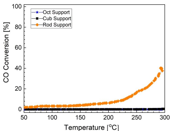
Figure S12. CO oxidation activity as a function of temperature over the three supports (CeO 2 octahedra, cubes and rods) after a 150 °C reduction treatment. Reaction conditions: CO=1.0 sccm, O 2 =10 sccm, Ar=10 sccm, He=79 sccm and heating rate 10 °C/min.
