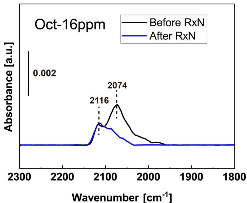
Figure S17. CO-DRIFTS data collected from Oct-16ppm after an in-situ exposure to CO oxidation conditions (CO=0.5 sccm, O 2 =5.0 sccm, He=44.5 sccm) at 283 °C inside the DRIFTS cell for 1 hour. After CO reaction, the catalyst was outgassed at 200 °C and cooled down in inert before being reduced at 150 °C (same procedure as for the fresh catalyst). Exposure of Oct-16ppm to the oxidative reaction conditions (excess oxygen), apparently reoxidized the Pt 0 species, while the non-reduced Pt δ+ species remain unaltered. It is expected that the Pt 0 atoms on the surface are very susceptible to reoxidation. These results further support the assignment of these species as single atoms. If Pt clusters were formed, more intense CO-DRIFTS peaks are expected as they would be more easily reduced compared with isolated Pt ions and the peaks would also shift to lower wavenumber. These experiments instead suggest that the single Pt 0 atoms have been converted to Pt δ+ species that are not reduced at 150 °C (or coordinatively saturated Pt δ+ species that does not adsorb CO) during these treatments. Unfortunately, the signal intensities cannot easily be compared between different runs as they are very sensitive to sample packing in the in-situ DRIFTS cell making quantitative comparisons difficult.
