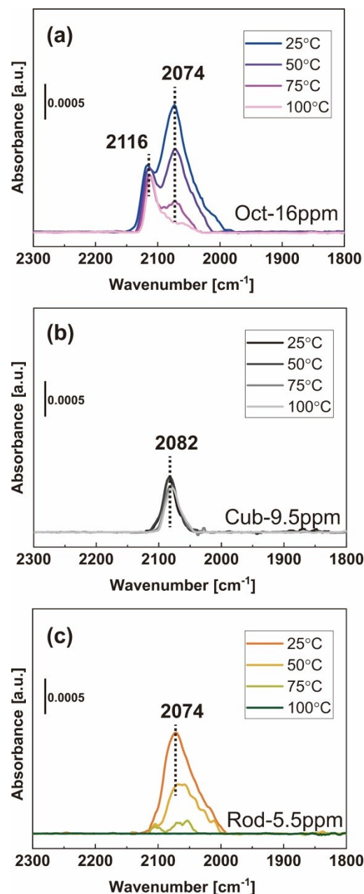
Figure 5 (a) CO-DRIFTS data collected from Oct-16ppm, Cub-9.5ppm and Rod-5.5ppm catalysts after reduction at 150 °C. All samples were purged under 20 sccm He flow at each temperature for 20 min.
