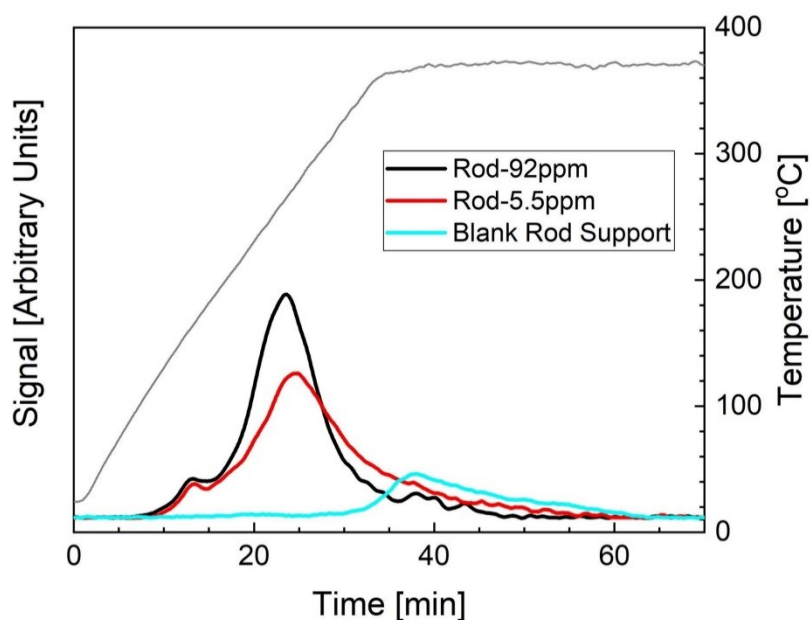
Figure S5. Temperature programmed reduction profiles collected from Rod-92ppm, Rod-5.5ppm and blank rod support. The corresponding temperature ramping file is shown in gray.
