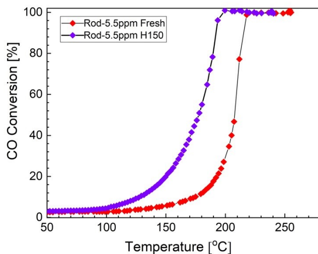
Figure S11. CO oxidation activity as a function of temperature over Rod-5.5ppm fresh (after calcination) and reduced at 150 °C. Reaction conditions: CO=1.0 sccm, O 2 =10 sccm, Ar=10 sccm, He=79 sccm and heating rate 10 °C/min.
