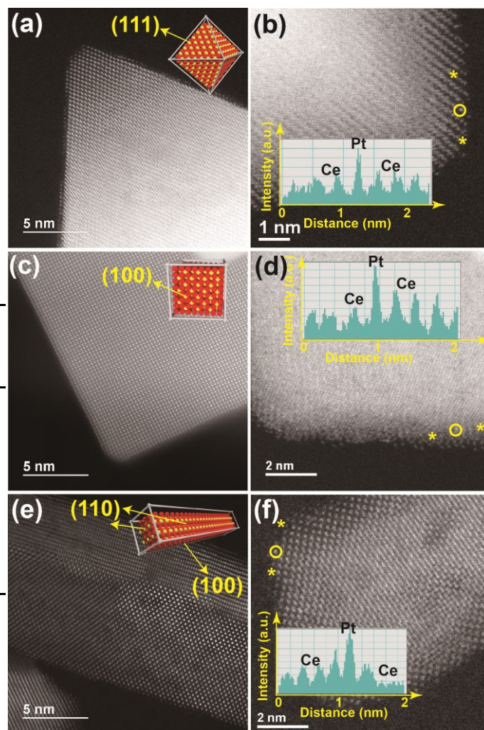
Figure 1 Atomic resolution HAADF-STEM images of (a) a \text{CeO}_2 octahedron obtained from a Pt/ \text{CeO}_2 -oct catalyst with a schematic of an octahedron exposing (111) surface facets, (b) fresh Oct-16ppm, (c) a \text{CeO}_2 cube obtained from a Pt/ \text{CeO}_2 -cub catalyst with a schematic of a cube exposing (100) surface facets, (d) fresh Cub-9.5 ppm, (e) a \text{CeO}_2 rod obtained from a Pt/ \text{CeO}_2 -rod catalyst with a schematic of a rod exposing (110) and (100) surface facets, and (f) fresh Rod-92 ppm. Yellow circles in ((b), (d), and (f)) indicate individual Pt atoms and insets display the line intensity profile along the line between two * symbols.
