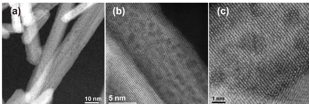
Figure S1. HR-STEM data at different magnifications obtained from CeO 2 nanorods. Vacancies and defects are visible as dark spots on the rods. The dark spots are evident on fresh as well as reduced rods. (a) and (b) Rod-5.5ppm after reduction at 150 °C. (c) Fresh Rod-92ppm.
