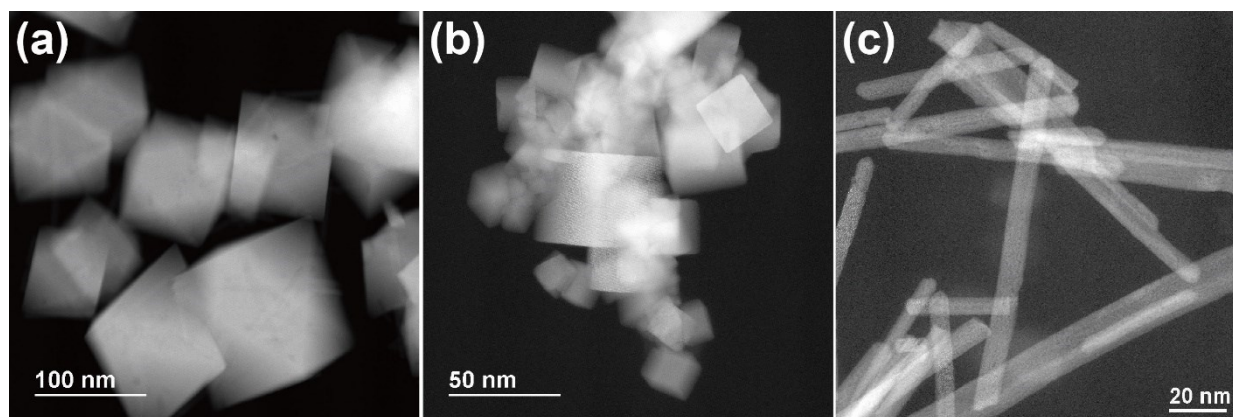
Figure S2. HAADF-STEM images of lower magnification to reveal that no Pt particles are observed after reduction at 150 °C. (a) Oct-6.5ppm, (b) Cub-9.5ppm catalyst, and (c) Rod-5.5ppm. Note that, when present, this resolution is sufficient to see Pt nanoparticles, as we have shown in our previous publication [60].
