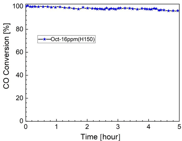
Figure S13. CO oxidation activity as a function of time at a temperature of 283 °C obtained over Oct-16ppm after a 150 °C reduction treatment in 5% H 2 . Reaction conditions: CO=1.0 sccm, O 2 =10 sccm, Ar=10 sccm, He=79 sccm.
