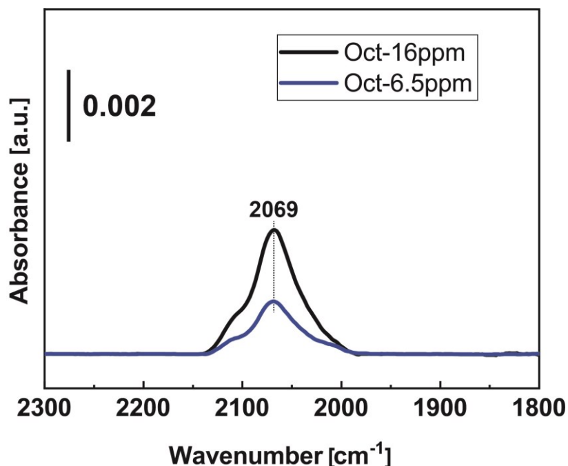
Figure S7. CO DRIFTS data collected from Oct-16ppm and Oct-6.5ppm after TPR experiments (reduction at 350 °C). After loading the catalysts into the DRIFTS cell, they were subjected to another reduction treatment at 200 °C to remove any oxygen that may have been adsorbed during sample transfer (flow of 5% H 2 (Airgas, UHP) and 95% Ar (Airgas, UHP) at 40 sccm for 30 minutes). After cooling to room temperature (25 °C) under a 40 sccm He flow, a background spectrum was collected. The catalysts were then exposed to CO at room temperature before data collection as described in the experimental section.
