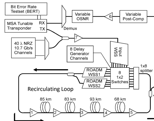
Fig. 1: Mesh network recirculating loop experiment [5] .
