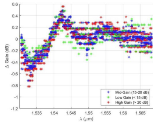
Fig. 3: Fully loaded gain ripple of six ROADMs amplifiers.
