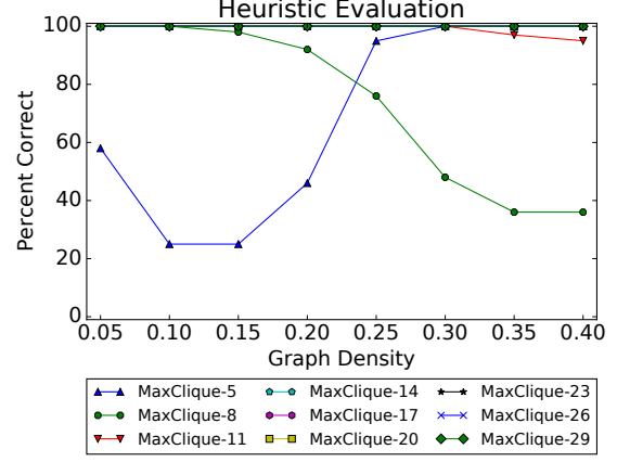
Fig. 4: Evaluation of the heuristic algorithm proposed in Algorithm 2. Individual lines denote the cardinality of the maximum clique inserted into the graph. The horizontal axis denotes the density of edges in the graph and the vertical axis denotes the percentage of test cases where the algorithm returned a clique of the correct cardinality. The heuristic algorithm returned cliques of the correct size 100 percent of the time for the graphs with max clique size of 14, 17, 20, 23, 26, and 29.
