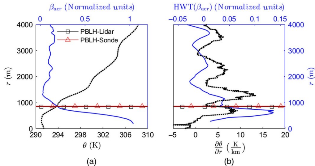
Fig. 5 A radiosonde launch with PBLH values found by lidar and radiosonde methods taken on March 13, 2021, 13:30 MST. (a) The aerosol backscatter coefficient (potential temperature) as the blue solid (black dotted) line. (b) The HWT (potential temperature lapse rate) as the blue solid (black dotted) line.
