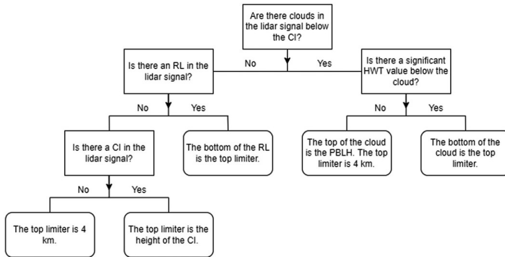
Fig. 2 A flowchart for determining the top limiter in the PBLH retrieval algorithm.
