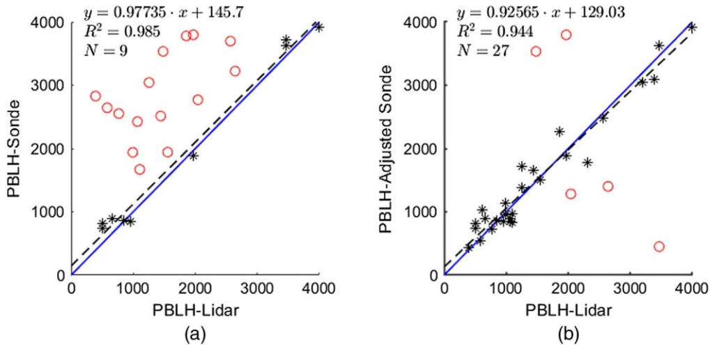
Fig. 8 Comparison between the lidar and radiosonde PBLH values. (a) A comparison between the HWT and Heffter PBLH values. The black asterisks represent sonde launches where the methods chose the same inversion layers as the PBLH, and the red circles represent sonde launches where the two methods chose different inversion layers as the PBLH. The black dotted line is a linear fit for the black asterisks, and the blue solid line is a 1 to 1 line for comparison. (b) The same as (a), except the lidar and adjusted radiosonde PBLH values are compared.
