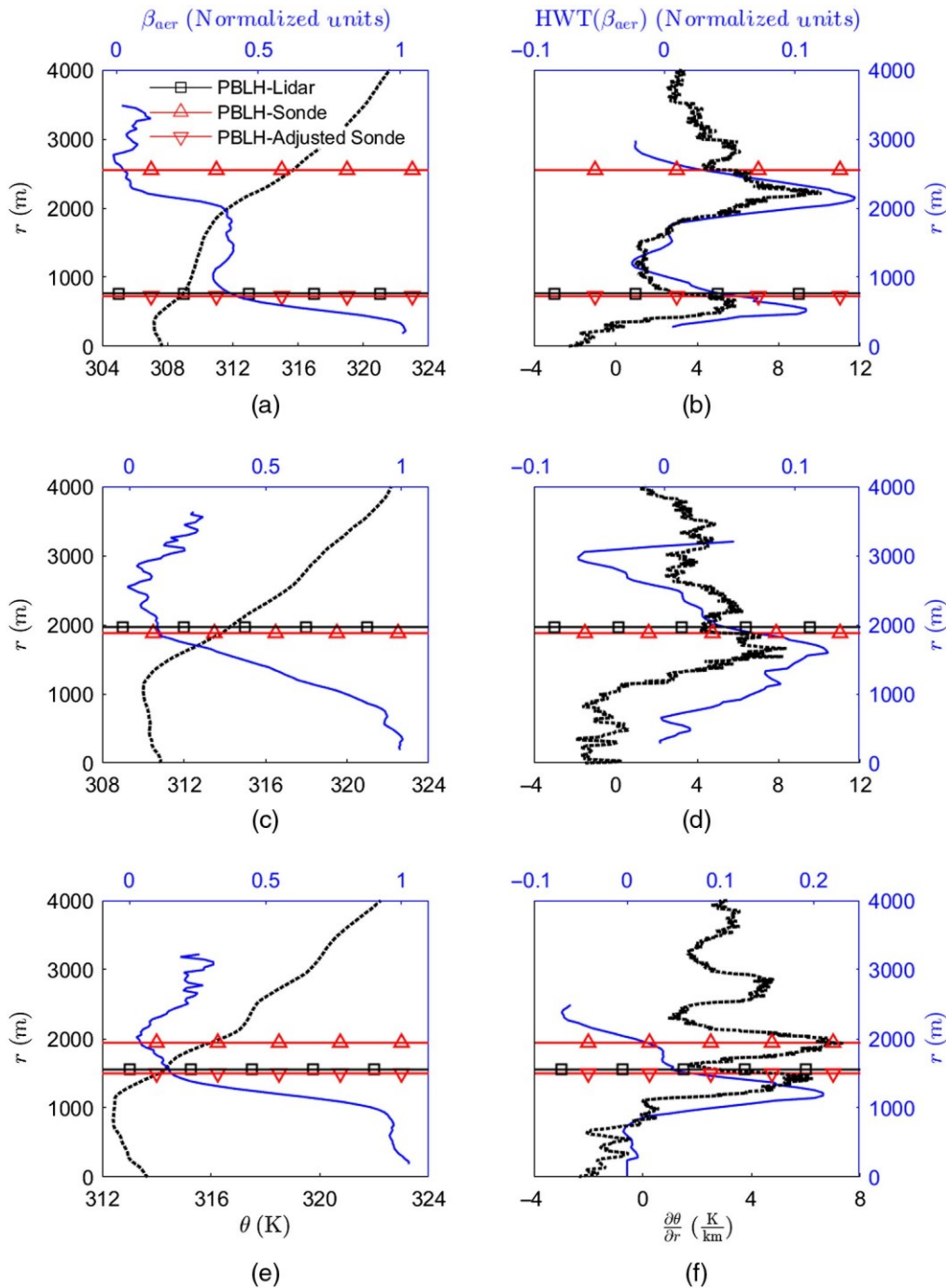
Fig. 7 Radiosonde launches with PBLH values found by lidar and radiosonde methods on June 2, 2021. (a) The aerosol backscatter coefficient (potential temperature) as the blue solid (black dotted) line for the sonde launched at 10:15 MDT. (b) The HWT (potential temperature lapse rate) as the blue solid (black dotted) line for the sonde launched at 10:15 MDT. (c) The same as (a) for the sonde launched at 12:49 MDT. (d) The same as (b) for the sonde launched at 12:49 MDT. (e) The same as (a) for the sonde launched at 15:32 MDT. (f) The same as (b) for the sonde launched at 15:32 MDT.
