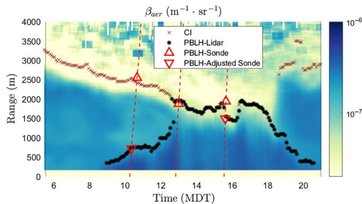
Fig. 6 The aerosol backscatter coefficient taken on June 2, 2021, with the PBLH and CI. The red-dashed lines represent radiosonde launches.
