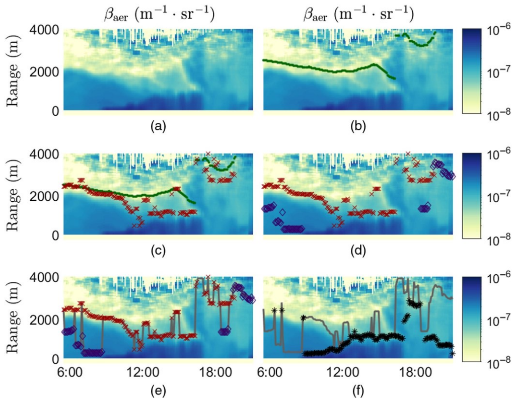
Fig. 3 The atmospheric layers found by the retrieval algorithm. (a) The aerosol backscatter coefficient on a logarithmic scale from sunrise to sunset. (b) The free atmosphere as green dots. (c) The CI as red crosses. (d) The bottom of RLs as purple diamonds. (e) The CI and RLs generate the top limiter, which is represented as a gray line. (f) The PBLH as black asterisks beneath the top limiter.
