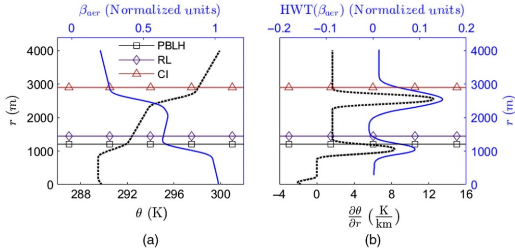
Fig. 1 The PBLH, RL, and CI for typical atmospheric conditions. (a) The aerosol backscatter coefficient (potential temperature) profile as a blue solid (black dotted) line. (b) The HWT of the aerosol backscatter coefficient (potential temperature lapse rate) as the blue solid (black dotted) line.
