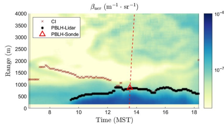
Fig. 4 The aerosol backscatter coefficient taken on March 13, 2021, from sunrise to sunset with the PBLH and the CI. The red-dashed line represents a radiosonde launch.
