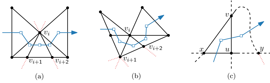
Fig. 14: For property (P3) in Lem. 9, observe that vertex v_i (which has degree 6) is (a) either open or (b) has a bend companion (here v_{i+1} ) with three ports; (c) for property (P4), note that two subsequent degree-4 vertices u and v cannot both be closed because of the two triangles they form with their common neighbors x and y .
