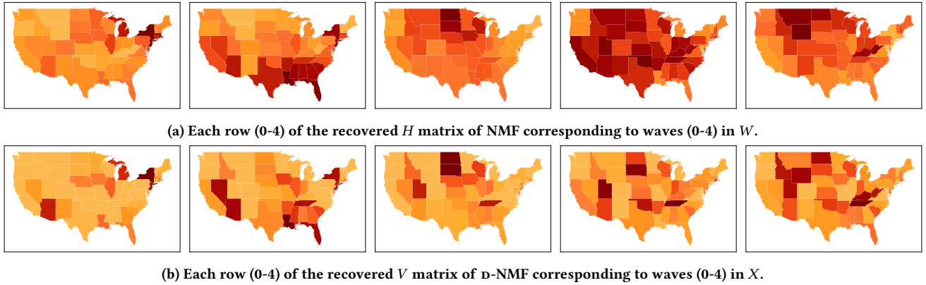
Figure 9: USA state-level coefficient matrices H , V recovered with NMF and d-NMF; large coefficients (i.e., darker colors) correspond to locations with high intensity for a given wave.
