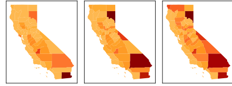
(b) Each row (0-2) of recovered V matrix of d-NMF corresponding to waves (0-2) in X .
