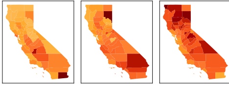
(a) Each row (0-2) of recovered H matrix of NMF corresponding to waves (0-2) in W .
