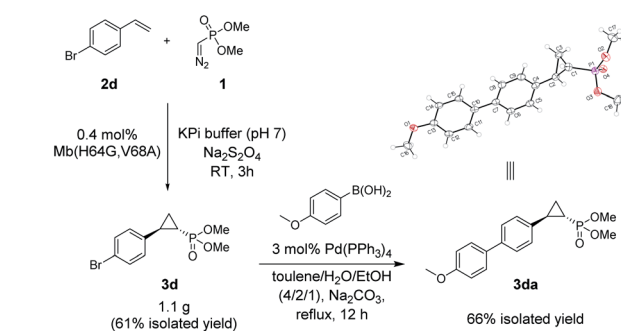
Scheme 1 Gram-scale biocatalytic synthesis of 3d and further functionalization to 3da for crystallographic analysis. See Fig. S5 and Table S8† for crystallographic data.
