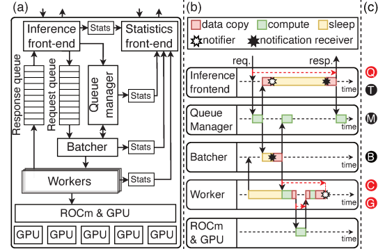
Figure 1: a) SCALESERVE design and components (Sec.2.1), b) Request/response life-cycle in SCALESERVE (Sec.2.2), c) Real-time statistics provided by each component (red circles correspond to the latency shown by the red arrows) (Sec.2.3).
