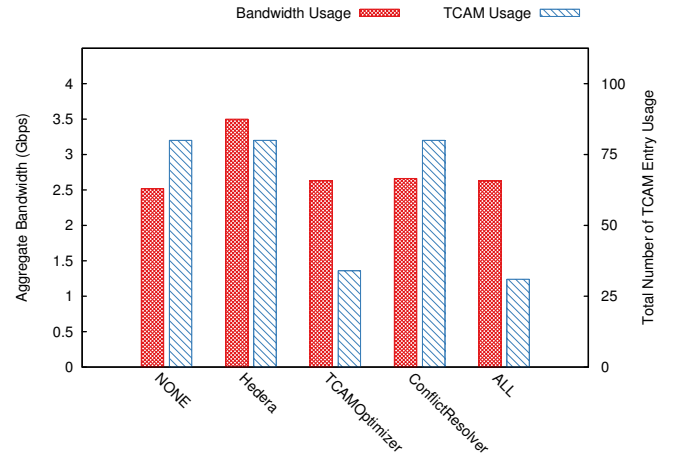
Figure 1: Aggregate Bandwidth and TCAM Usage.
