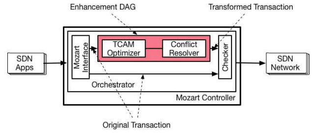
Figure 2: Re-Designed SDN Controller.
