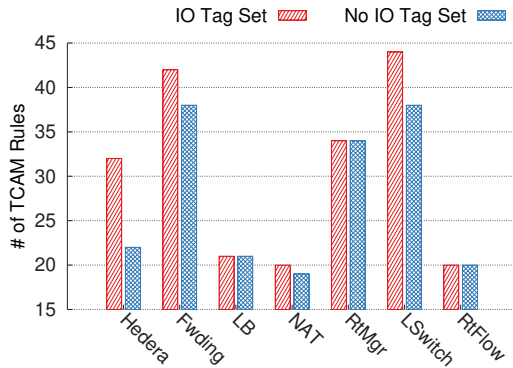
Figure 6: Number of TCAM Entries when {IO} is Enabled.
