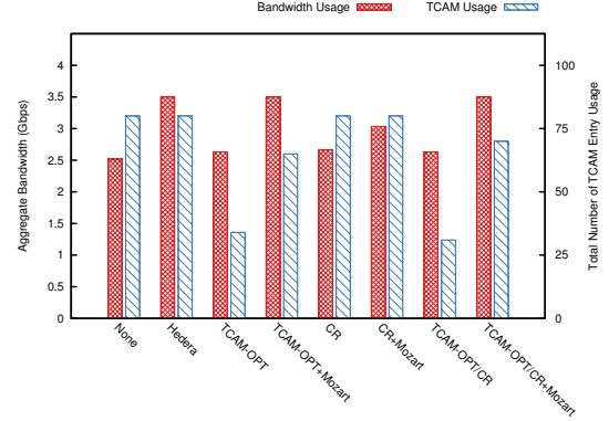
Figure 7: Aggregate Bandwidth and TCAM Usage.
