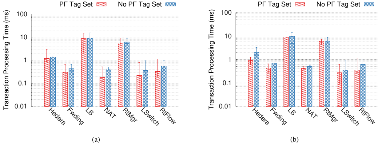
Figure 5: (a) {PF} SDN-Flags' Impact on Transaction Processing Time. (b) {PF} SDN-Flags' Impact with Multiple Simultaneous SDNApps.
