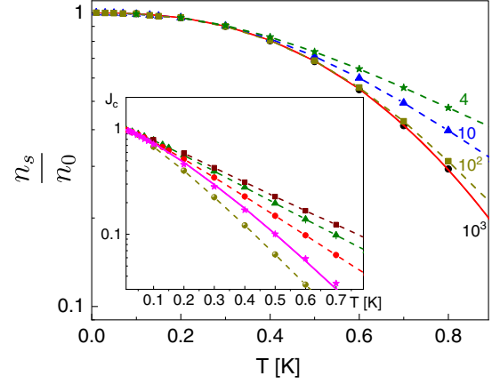
FIG. 5. Superfluid density n_s (dashed lines are guides to the eye) for linear sizes \tilde{L} specified next to each dataset. The solid line is the fit by \exp[-(T/T_a)^\alpha] , with \alpha = 5/2 and T_a = 0.737 \pm 0.005 . Inset: the critical current J_c (normalized to unity at T = 0 ) for \tilde{L} = 4, 10, 10^2, 10^3, 10^4, 10^7 increasing from the highest to the lowest dataset. The solid line is the fit of the \tilde{L} = 10^4 data by J_c \propto \exp[-(T/T_a)^{5/4}] , with T_a = 0.257 \pm 0.01 . All data for J_c are consistent with \alpha \approx 5/4 \pm 0.1 for 0 < T < 0.6 and the spread is due to T_a varying by a factor \sim 2 (cf. Fig. 1).
