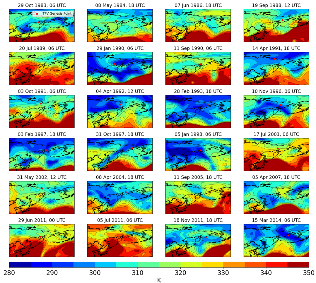
Figure A2. Maps of tropopause potential temperature (K; fill and contours) 12 h prior to each TPV genesis event in the eastern Siberia non-likely split cluster. Red dots indicate the eventual genesis location of the TPV.
