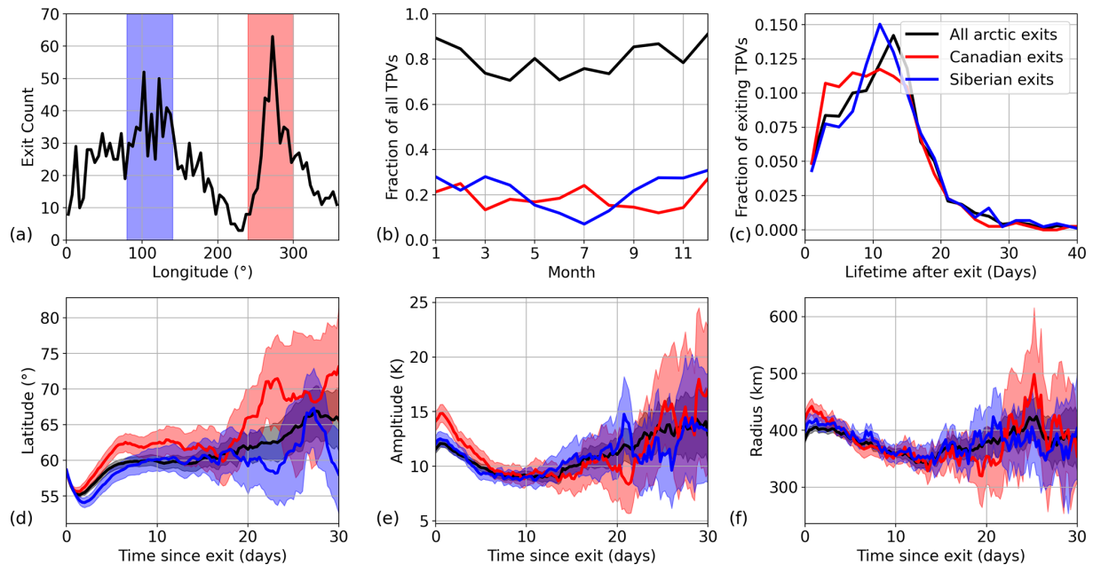
Figure 13. (a) Line histogram of longitudes (°) at which long-track TPVs exited the Arctic (crossed 60° N) for the first time. Blue shading represents the range of cases included in the Siberian exit maximum (80–140°), and red shading represents the Canadian exit maximum (240–300°). (b) The fraction of all long-track TPVs that exited the Arctic at any point by month of exit (black), along with the fraction of these TPVs that exited via the Siberian (blue) and Canadian (red) pathways. (c) Lifetime (days) of all exiting long-track TPVs (black), Siberian exits (blue), and Canadian exits (red) after exiting the Arctic. (d) Average latitude (°) of post-exit TPVs for all exits (black), Siberian exits (blue), and Canadian exits (red). Shading represents confidence at the 95 % level established with bootstrap resampling tests. (e) As in (d), but for average TPV amplitude (K). (f) As in (d), but for average TPV radius (km).
