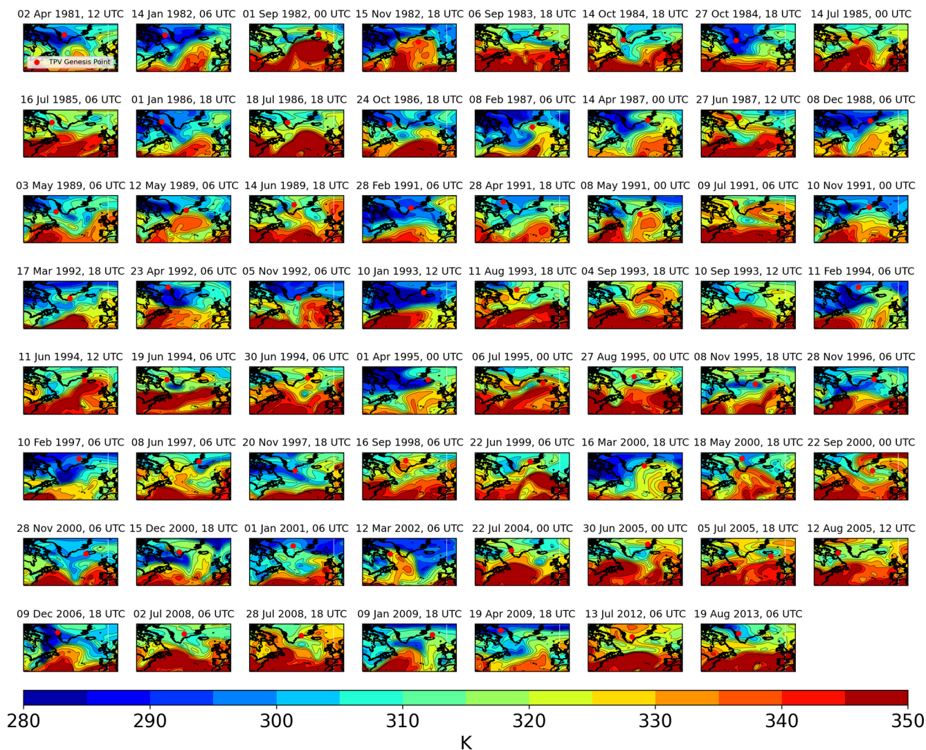
Figure A4. Maps of tropopause potential temperature (K; fill and contours) 24 h prior to each TPV genesis event in Greenland non-likely split cluster. Red dots indicate the eventual genesis location of the TPV.
