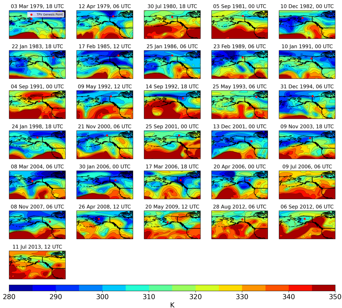
Figure A8. Maps of tropopause potential temperature (K; fill and contours) 12 h prior to each TPV genesis event in the Alaska non-likely split cluster. Red dots indicate the eventual genesis location of the TPV.
