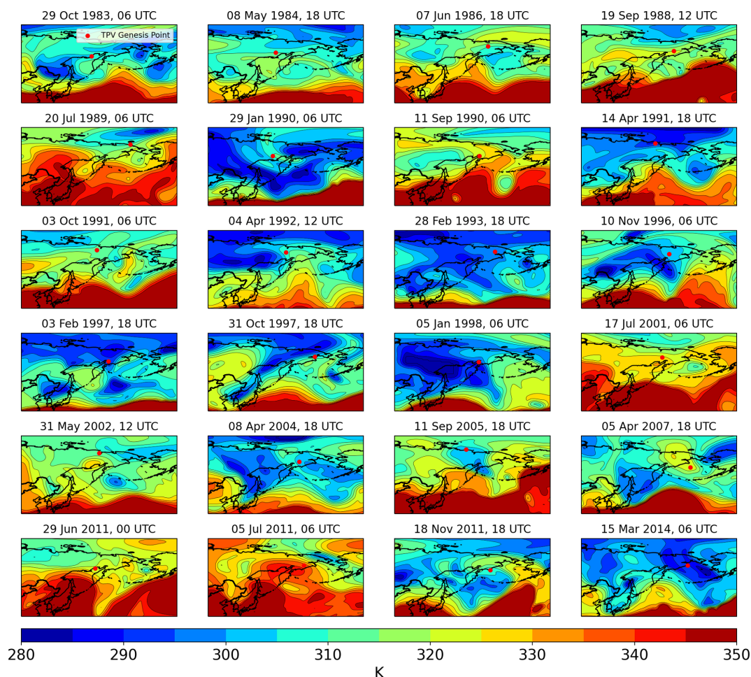
Figure A1. Maps of tropopause potential temperature (K; fill and contours) 24 h prior to each TPV genesis event in the eastern Siberia non-likely split cluster. Red dots indicate the eventual genesis location of the TPV.
