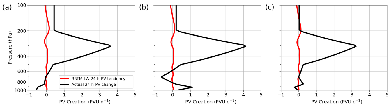
Figure 9. (a) Vertical profiles of true change in PV over the 24 h preceding TPV genesis (black; \text{PVU d}^{-1} ) and calculated change in PV during this time based on longwave heating and cooling from water vapor (red; \text{PVU d}^{-1} ) averaged across all cases in the eastern Siberia non-likely split cluster. Expected changes in PV due to longwave heating and cooling are calculated using single-column RRTM-LW with the average humidity and temperature profiles through the location of TPV genesis, 24 h before the genesis event (i.e., a profile through the center of Fig. 8a). (b) As in (a), but for the Greenland non-likely split cluster. (c) As in (a), but for the Alaska non-likely split cluster.
