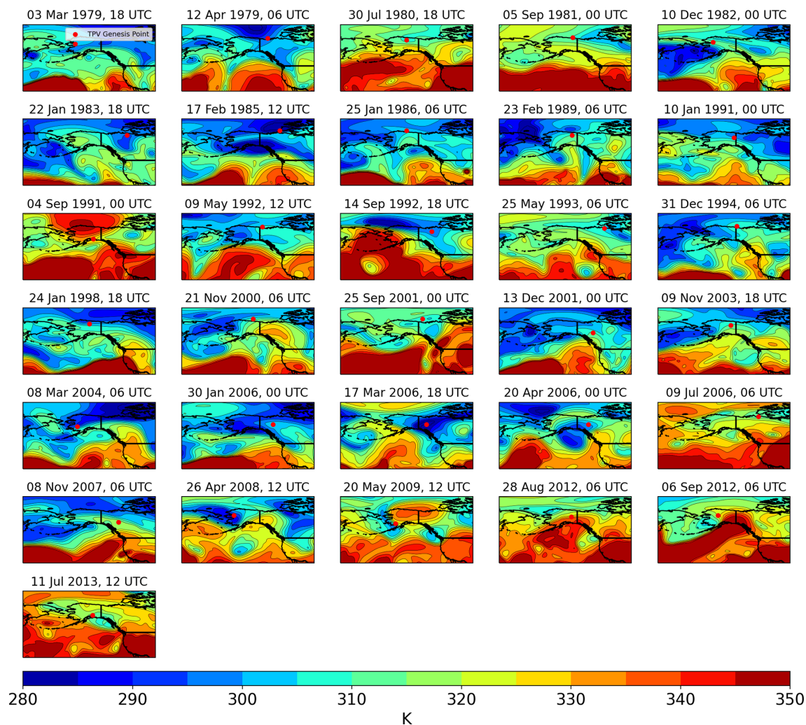
Figure A7. Maps of tropopause potential temperature (K; fill and contours) 24 h prior to each TPV genesis event in the Alaska non-likely split cluster. Red dots indicate the eventual genesis location of the TPV.
