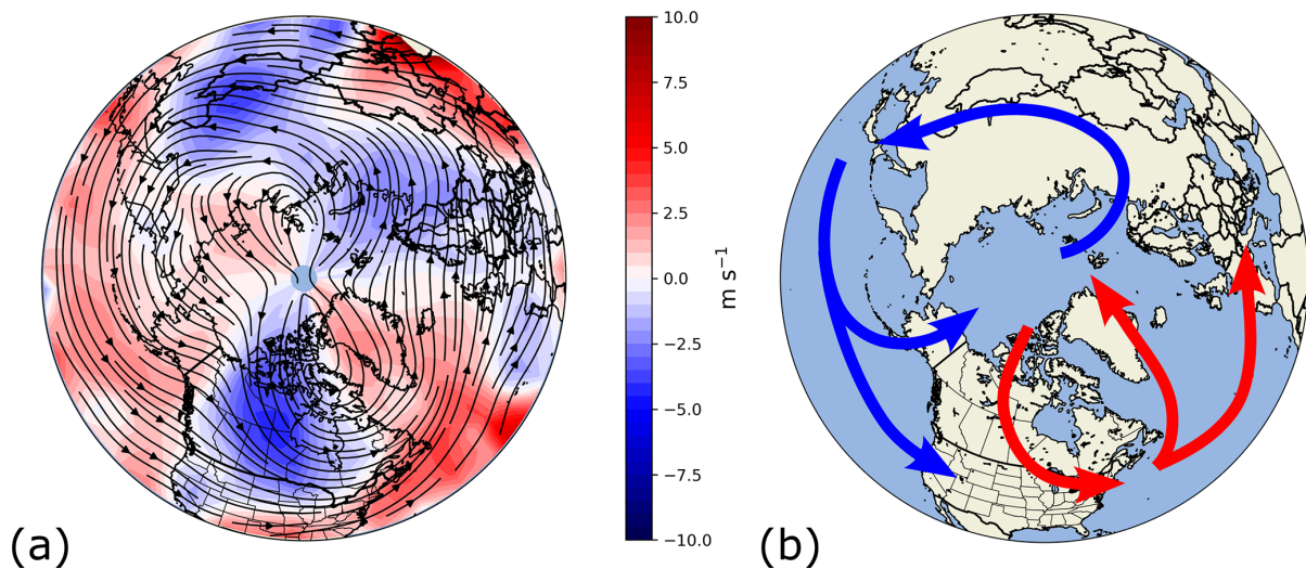
Figure 14. (a) Streamlines (black) of average long-track TPV motion and average meridional TPV speed ( \text{m s}^{-1} ; fill), calculated as vector averages within 5° by 5° latitude–longitude bins. (b) Schematic of the Siberian (blue) and Canadian (red) Arctic exit, transport, and reentry pathways observable in (a) and in Fig. 11
