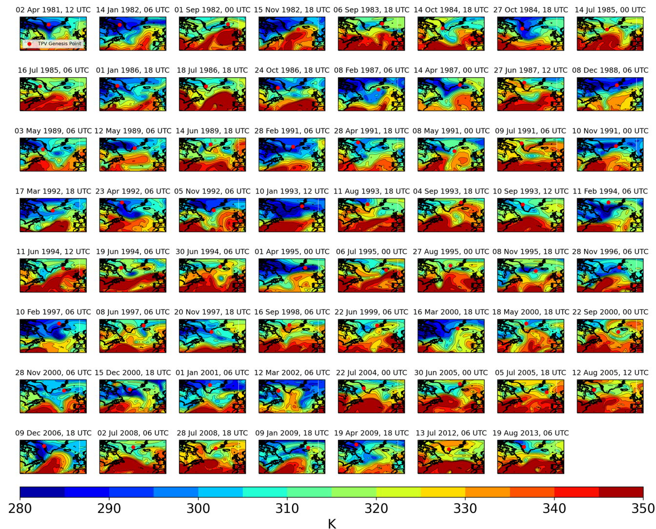
Figure A5. Maps of tropopause potential temperature (K; fill and contours) 12 h prior to each TPV genesis event in the Greenland non-likely split cluster. Red dots indicate the eventual genesis location of the TPV.
