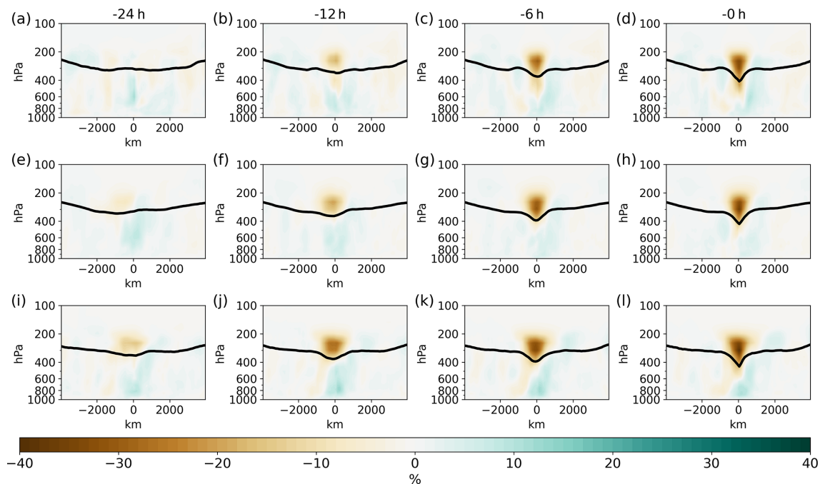
Figure 8. Rotationally averaged cross-section composites of relative humidity anomaly (%; fill) through the genesis points of all TPVs within the eastern Siberia non-likely split cluster at (a) 24 h before TPV genesis, (b) 12 h before TPV genesis, (c) 6 h before TPV genesis, and (d) the time of TPV genesis. The 2 PVU surface (hPa) is included on each panel as a solid black line. (e–h) As in (a)–(d) but for the central Greenland non-likely split cluster. (i–l) As in (a)–(d) but for the northern Alaska non-likely split cluster.
