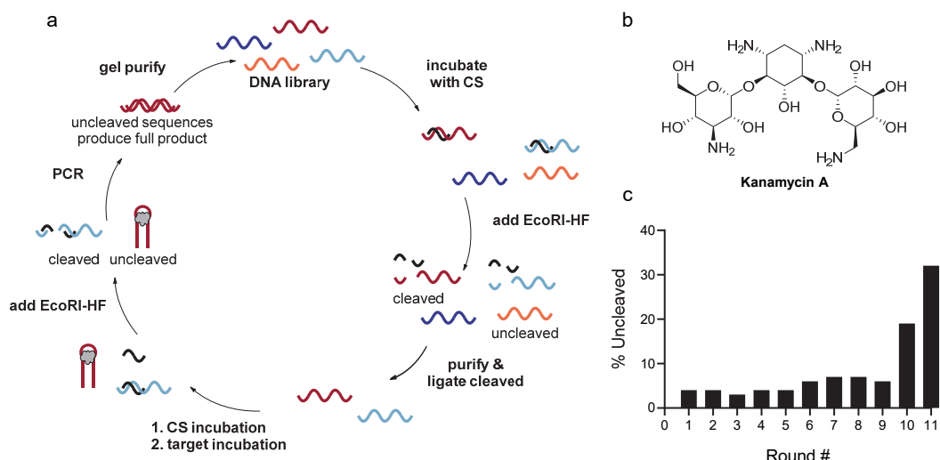
Figure 2. Homogenous EcoRI-HF SELEX to generate structure-switching aptamers. (a) FAM-labelled DNA library having an N_{40} random region was hybridized to capture strand and the complex digested with EcoRI-HF. The cleaved product (70 nt) was gel purified and full-length product (90 nt) was recovered through split ligation by T4 DNA ligase. The re-ligated library members were hybridized to free capture strand and incubated with the target. Active biosensor sequences were enriched by EcoRI-HF digestion followed by PCR amplification. ssDNA library was purified by 10 % denaturing PAGE and carried on to subsequent selection rounds. (b) Chemical structure of kanamycin A. (c) Progression of EcoRI-HF SELEX to generate structure-switching aptamers to kanamycin A. Following digestion, cleavage products were monitored by 10 % denaturing PAGE. Band intensity was used to quantify percent uncleaved.
