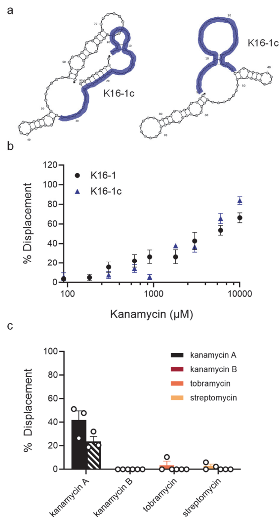
Figure 4. K16-1 and K16-1c function as structure-switching aptamer sensors and are specific to kanamycin A. (a) Secondary structure of K16-1 with (left) and without (right) the 9 nt capture strand calculated using NUPACK. The K16-1c truncation is highlighted in purple with (left) and without (right) the 9 nt capture strand calculated using NUPACK. (b) Capture strand displacement as a function of kanamycin A concentration with 100 nM K16-1 and 500 nM K16-1c with 100 nM and 125 nM 9 nt capture strand, respectively. Samples resulting in negative displacement were denoted 0% displacement. Error bars denote standard error ( n=9 ). (c) Displacement of K16-1 (solid) and K16-1c (dashed) biosensors with 1000 \mu\text{M} kanamycin A, kanamycin B, streptomycin, or tobramycin. Error bars denote standard error ( n=3 ).
