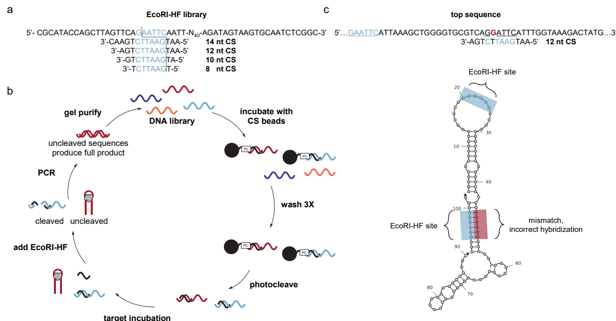
Figure 1. Bead assisted EcoRI-HF SELEX to generate structure-switching aptamers. (a) EcoRI-HF library and capture strand sequences with recognition sites in blue. Cut site is illustrated by dotted line. (b) FAM-labelled DNA library having an N 40 random region was hybridized to immobilized capture strand and the complex washed and photocleaved. After target incubation, bound sequences were recovered following EcoRI-HF digestion and PCR amplification. Gel purified library was then carried on to subsequent rounds. ssDNA library was purified by 10% denaturing PAGE and carried on to subsequent selection rounds. (c) Highly enriched sequences did not correctly hybridize the capture strand through the built in EcoRI-HF recognition site (underlined blue) Sequences containing partial recognition sites in the N40 region (underlined black) with one or more mismatches (red, bold) were present in predicted structures by NUPACK.
