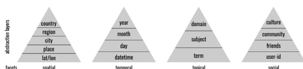
Figure 4. Abstraction layers for each facet (Löchner, Dunkel, Burghardt, 2018).
