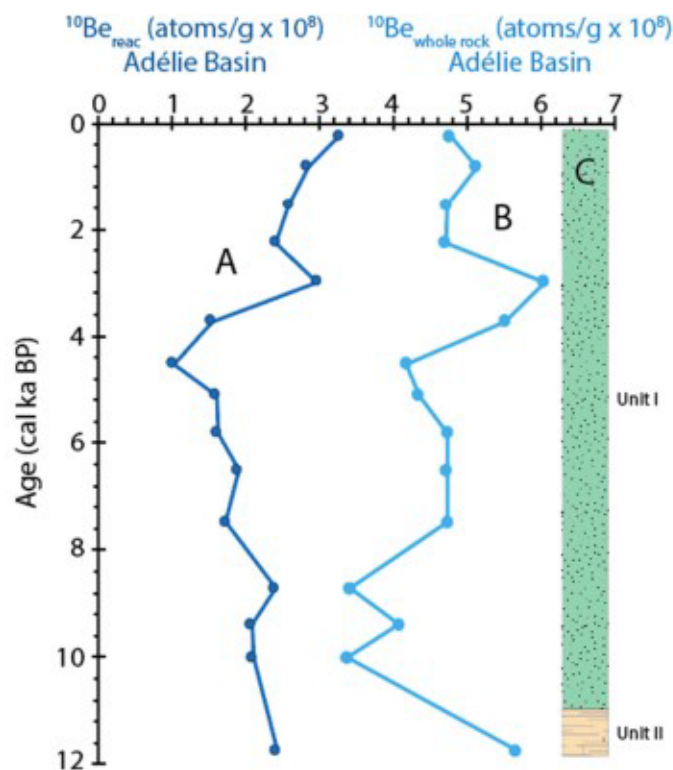
Fig. 4. Results of Adélie Basin ^{10}\text{Be}_{\text{reac}} from (A) this study, (B) whole rock ^{10}\text{Be} results from Behrens et al. (2019), and (C) lithology of hole U1357A.
