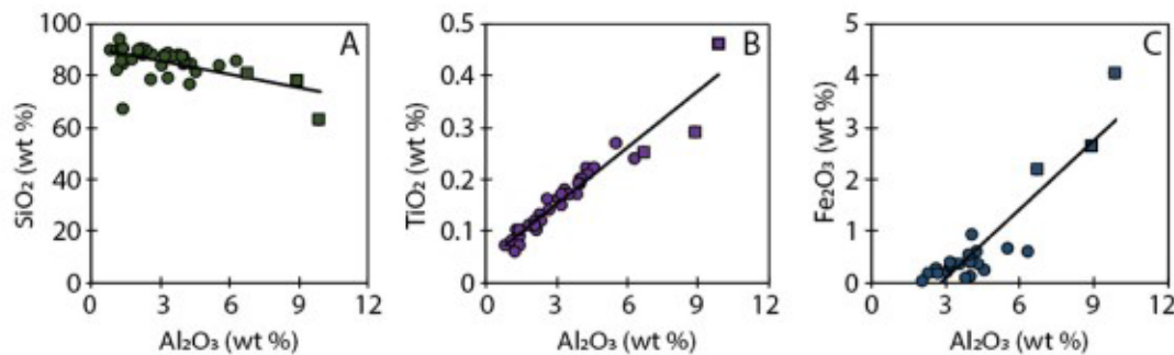
Fig. 3. Scatter plots of Adélie Basin A) \text{SiO}_2 vs. \text{Al}_2\text{O}_3 ; B) \text{TiO}_2 vs. \text{Al}_2\text{O}_3 ; C) \text{Fe}_2\text{O}_3 vs. \text{Al}_2\text{O}_3 . The squares in each plot correspond to the same three bottom-most samples where the highest amount of terrigenous input was observed in the sediment core.
