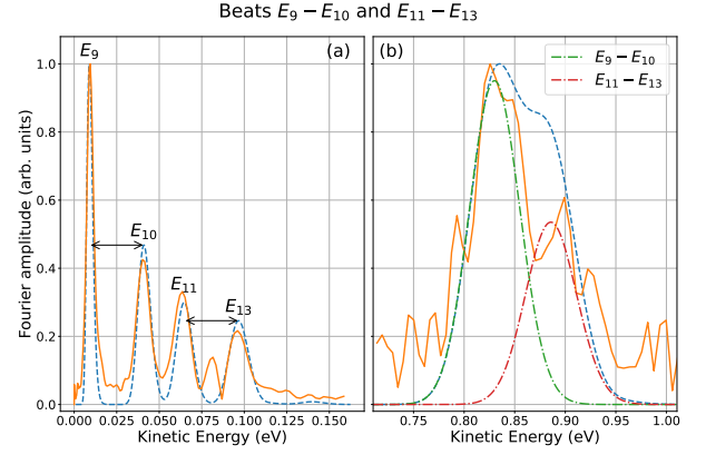
FIG. 4. (a) Kinetic energy resolved amplitude of difference autoionization signal in experiment (solid line) and theory (dashed line) differentiates two beat pairs, between states 9 f' and 10 f' and states 11 f' and 13 f' , that lie in the same beat frequency bin and otherwise would be non-separable. (b) Photoionization spectra do not have the kinetic energy resolution to distinguish the overlapping contributions in experiment (solid line) or theory (dashed line). Calculated photoionization amplitude for each beat pair is shown (dot-dashed line).
