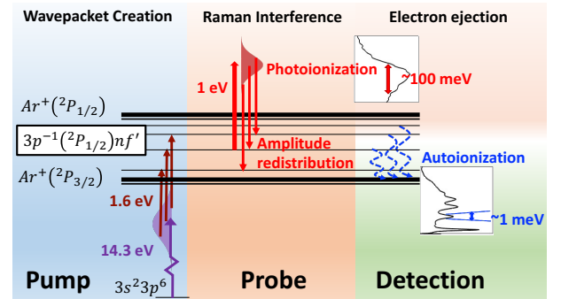
FIG. 1. Two color (EUV+NIR) ‘pump’ pulse excites an nf' autoionizing wavepacket in the argon atom. A time-delayed femtosecond SWIR ‘probe’ pulse induces impulsive Raman transitions between the constituents of the wavepacket, redistributing the population within the wavepacket. Electronic states undergo slow autoionization producing sharp features in the electron spectra. Analysis of changes in the spectra of this delayed signal as function of pump-probe delay provides both time and energy resolution.
