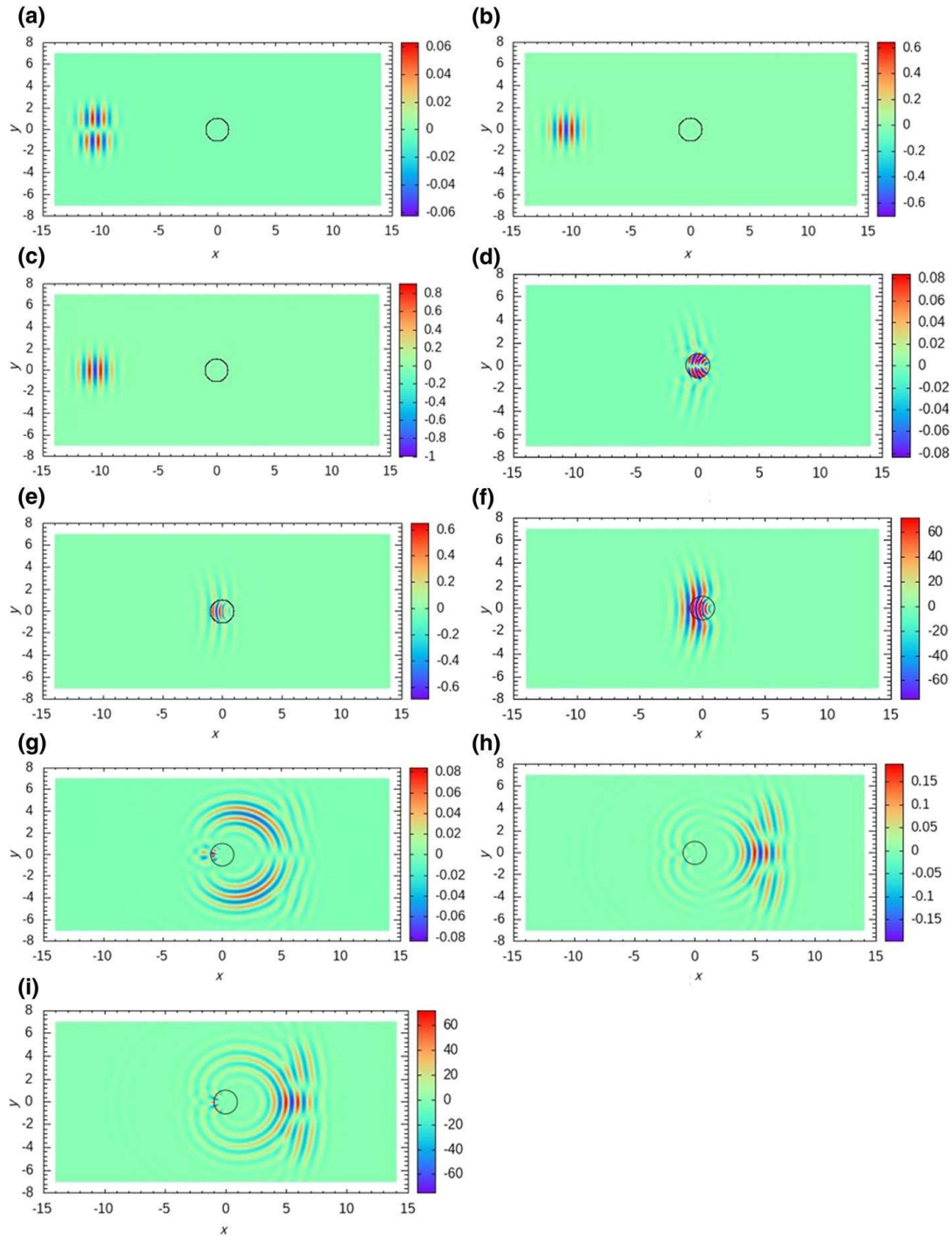
Fig. 12 Solution variables Dx , Dy , and Bz for the test problem shown in Fig. 11. We used a second-order scheme with a 2880 \times 1440 zone mesh. At that resolution, any further change in the solution becomes indistinguishable by eye. The solution on this mesh was used as a reference solution for all our second-order runs. Similar third and fourth order simulations were used as reference simulations for our third and fourth order tests. a–c Solution variables at time 0. d–f Solution variables at 3.5 \times 10^{-8} s, at which time the wave is interacting strongly with the refractive disk. g–i Show the solution variables at 5.7 \times 10^{-8} s, by which time the Gaussian pulse has scattered off the refracting cylinder. The black circle shows the extent of the disk with a radius of unity
