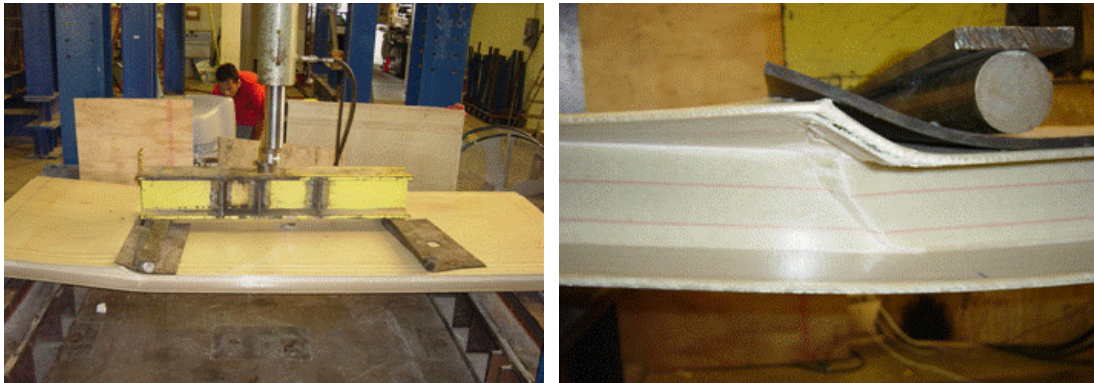
Fig. 14. Four point bending with a span of 100'' for 48'' x 120'' GFRP panel
