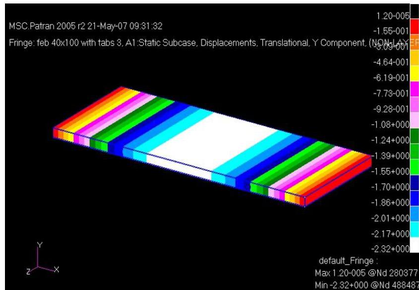
Fig. 18. Deflection contours Predicted by 3D orthotropic solid model for 40"x100" CFRP panel
