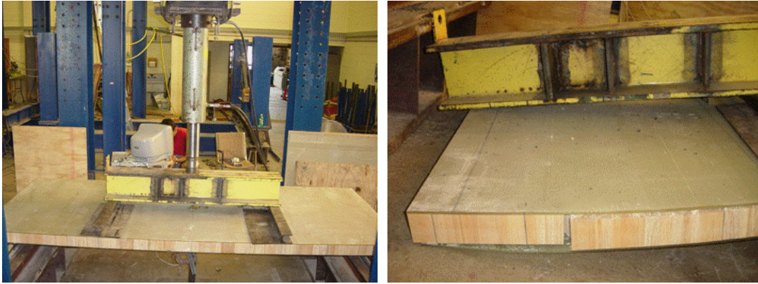
Fig. 8. 3.5" VARTM panel (4' x 10', provided by NGSS) being tested to failure with exposed cracking
