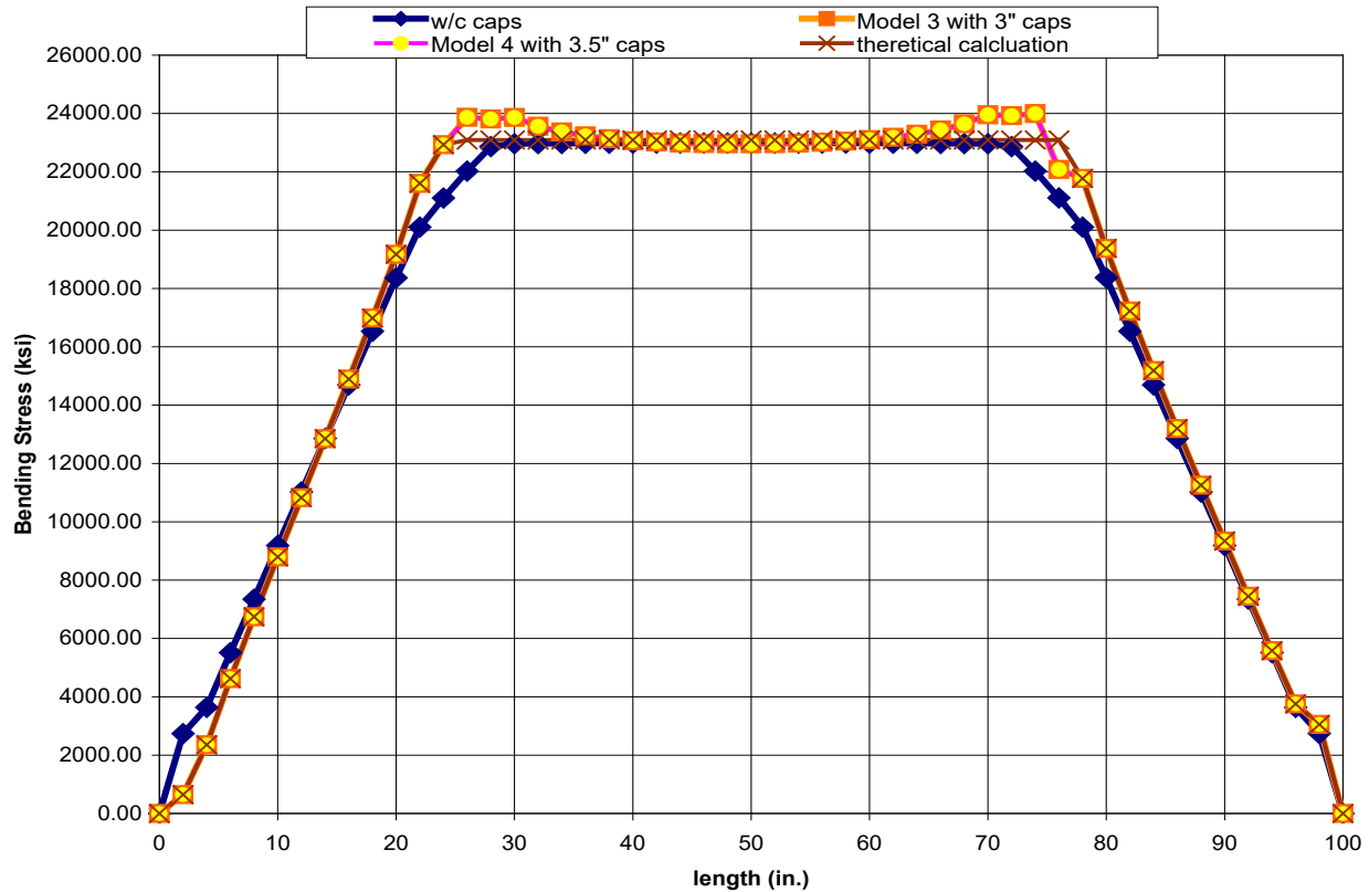
Fig. 17. Predicted bending stress across the span for 40"x100" x3.5" CFRP panel
