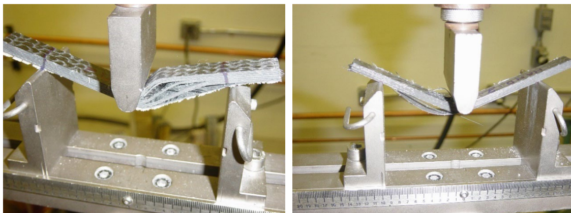
Fig.12. Typical failed bending specimens for carbon /VE (left) vs. carbon/epoxy (right)
