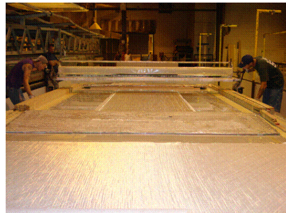
2) Applying resin for impregnation
