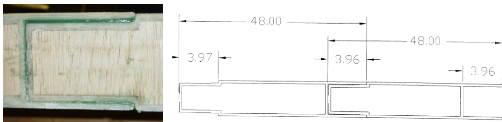
Fig. 5. A double sided lap joint and schematic joining of two 4' wide modular panels (units in inches)
