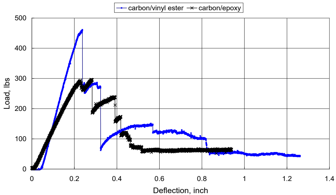
Fig. 11. Typical bending load versus deflection curve for carbon / VE vs. carbon/Epoxy (@ 3Pt Bending)
