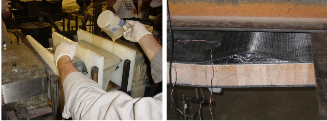
Fig. 4. Poor adhesion between carbon and vinyl ester leading to wet out problem during manufacturing (left) and interlaminar failure (right)
