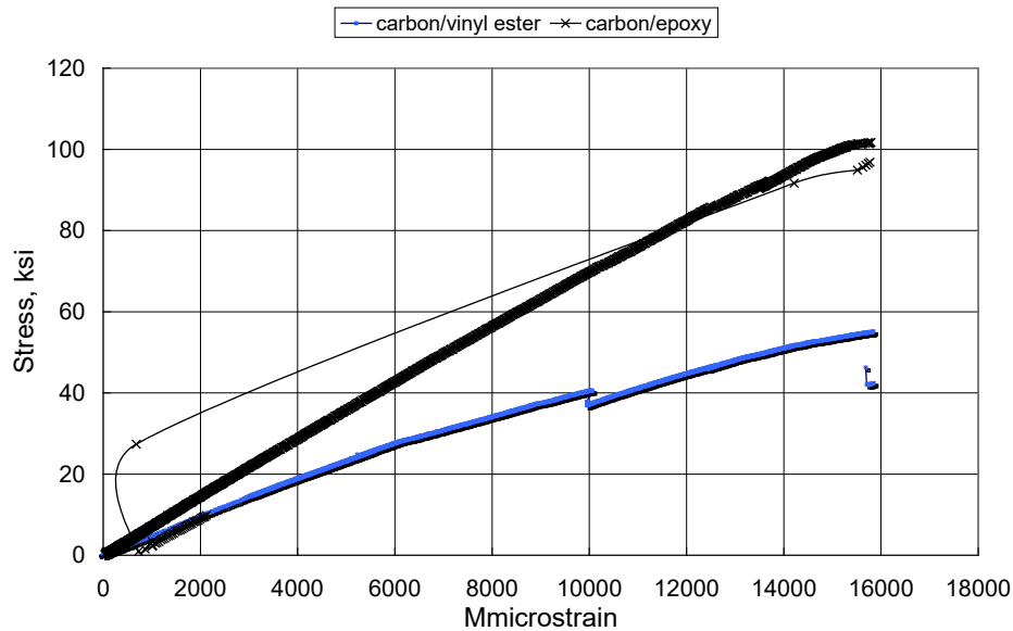
(a) Carbon/Vinyl Ester vs Carbon/Epoxy: Typical Stress VS Strain @ Tension
