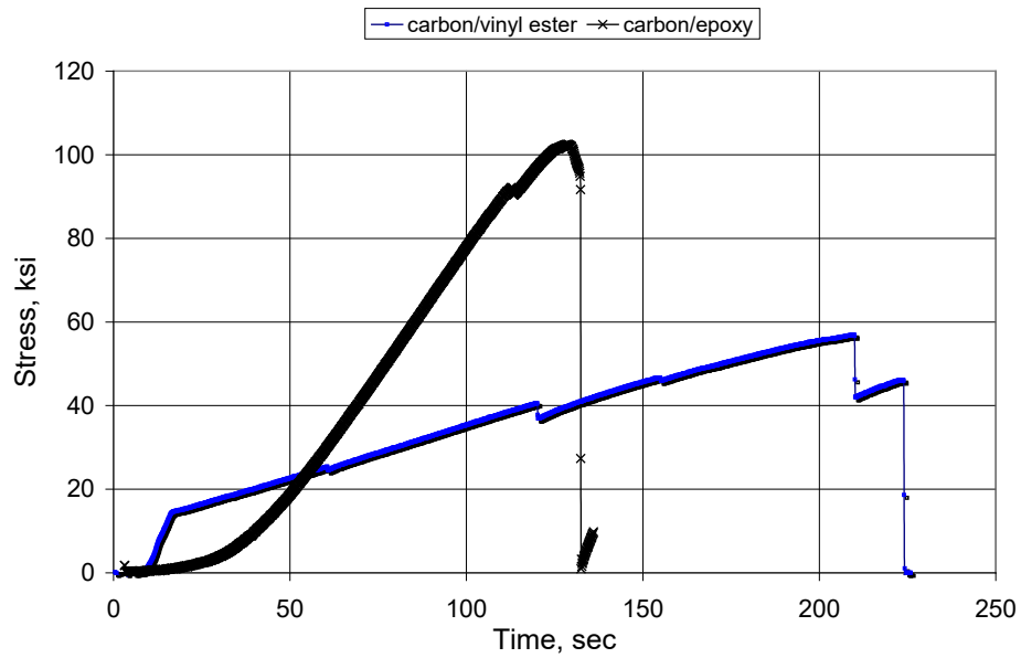
(b) Carbon/Vinyl Ester vs Carbon/Epoxy: Typical Stress VS Time @ Tension
