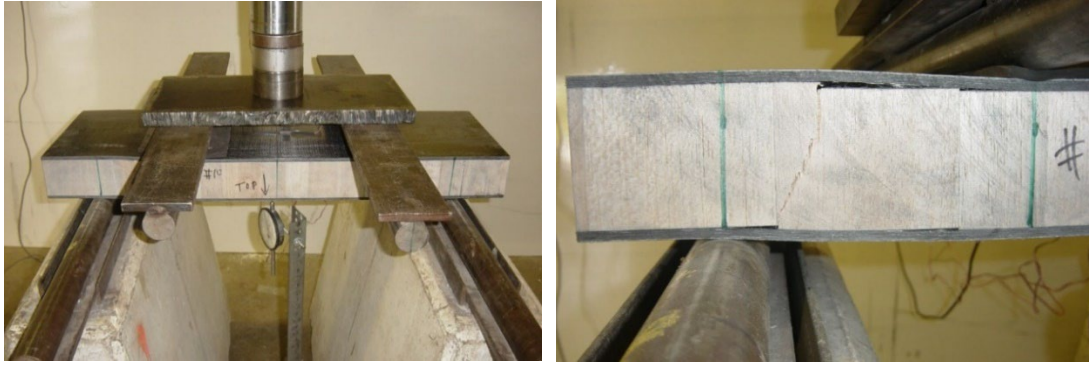
Fig. 13. Four point bending (short beam shear) with a span of 27'' for 12'' x 36'' CFRP sample
