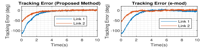
Fig. 2. Plots of tracking error (deg) versus time (s) in presence of AWG measurement noise with the proposed method and e-mod.
