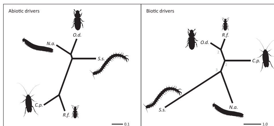
Fig. 2. Unrooted dendrograms representing two competing hypotheses about key drivers of phylogeographic congruence among five saproxylic invertebrates: abiotic factors related to historical climatic stability (left) versus biotic factors related to ecological co-associations (right). Scale bars represent either the inverse of a measure of habitat overlap (1 – Schoener’s D ; left), or the cumulative dissimilarity score for species interactions based on trophic guild, timing of colonization during succession, frequency of syntopy, and presumed interaction type (right). Numbers on nodes for the biotic drivers scenario indicate the number of jackknife replicates (out of 4) that supported a given predicted partition. Species names are abbreviated as in Fig. 1.
