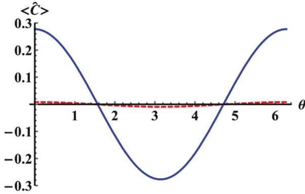
FIG. 6. Quantum interference between the two components of a Schrödinger cat state. The blue (solid) curve shows the expectation value of operator \hat{C}_j(0, \Delta) as a function of \theta evaluated before the beam splitter. The red (dashed) curve shows the expectation value of \hat{C}_j(0, \Delta) after the beam splitter using the same parameters as in Fig. 5(b). It can be seen that passing a Schrödinger cat state through a beam splitter will reduce the quantum interference by an amount that is much larger than the reduction in the field amplitude [42]. (Arbitrary units.)
