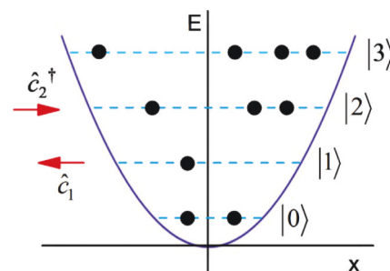
FIG. 2. A harmonic oscillator potential containing N identical bosons represented by black dots. The operators \hat{c}_n^\dagger and \hat{c}_n create or annihilate a particle in the oscillator potential in state |n\rangle . The field operator \hat{\psi}^\dagger(x) creates a particle at coordinate x . In the case of the electromagnetic field, these hypothetical particles will be referred to as oscillatons.
