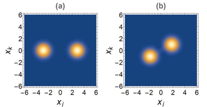
FIG. 5. Joint probability density P_j(x_j, x_k, t) for a Schrödinger cat state plotted as a function of the quadratures x_j and x_k . (a) Joint probability distribution evaluated before the beam splitter ( t = 0 ). (b) Entangled state produced by the beam splitter [12] with \varepsilon = 0.12 and t = 12 . (Arbitrary units.)
