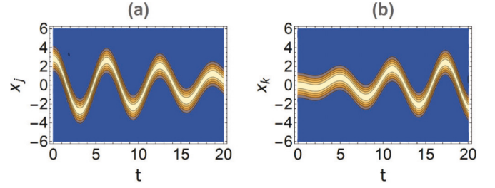
FIG. 4. Effects of a beam splitter on a coherent state incident in mode j with mode k initially in its vacuum state. (a) Probability density P(x_j, t) = \langle \hat{\psi}_j^\dagger(x_j, t) \hat{\psi}_j(x_j, t) \rangle for mode j plotted as a function of the quadrature x_j and the time t . (b) Probability density P(x_k, t) for mode k . The width of these probability distributions is due to vacuum fluctuations. (Arbitrary units.)
