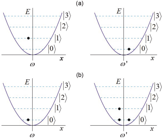
FIG. 8. Initial (a) and final (b) states of interest in the photon scattering experiment of Fig. 7. Each of the drawings represents the harmonic oscillators that corresponds to modes of the electromagnetic field with angular frequency \omega or \omega' . The black dots show the energy levels occupied by the oscillators in each mode.
