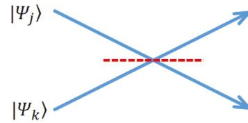
FIG. 3. Two beams of light incident on a beam splitter.
