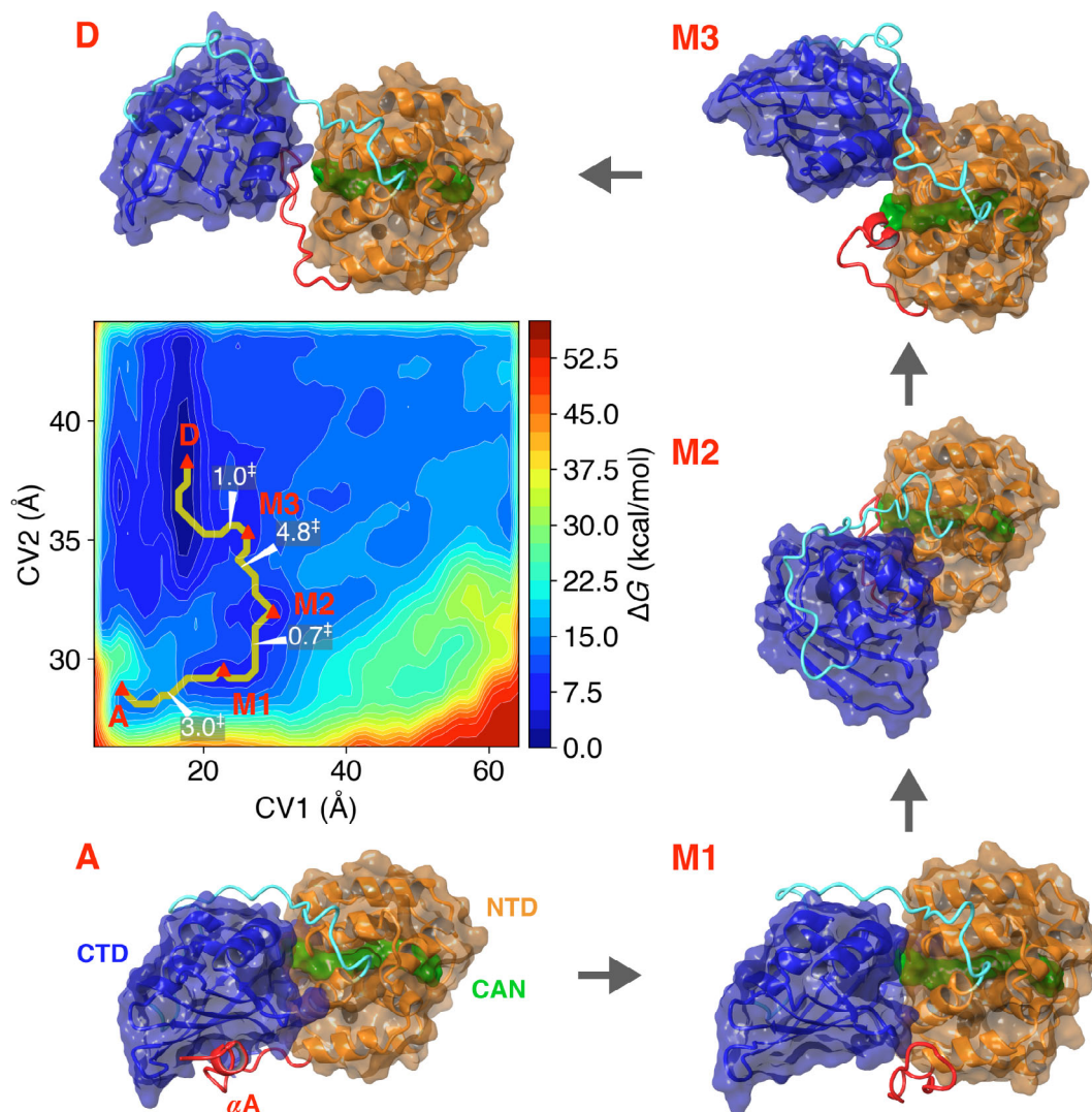
FIGURE 3 Minimum free energy path (MFEP) of the OCP-P3 domain dissociation. The molecular-surface representations correspond to the common configuration in the states labeled on the free energy surface. On the FES, the wedges denote free energy barriers in units of kcal/mol; the yellow line represents the MFEP
