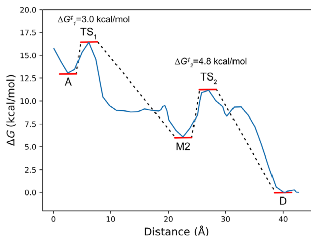
FIGURE 4 Free energy barriers along the MFEP of the OCP-P3 domain dissociation. A, the associated state; M2, a metastable state; D, the dissociated state; TS 1 and TS 2 , transition states
