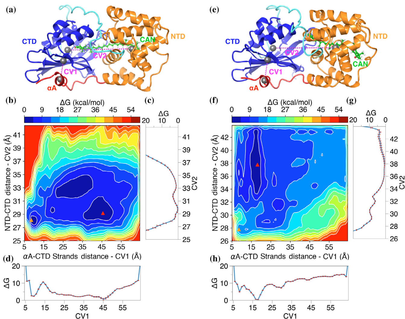
FIGURE 1 The resulting free energy surfaces from WT-metaD simulations of domain separation starting from OCP O (left panel) and OCP-P3 (right panel). Molecular representations of OCP O (a) and OCP-P3 (e). The CVs represent the distances between the centers of mass (COM, grey spheres) of different segments of OCP. CV1 represents the distance between the COM of the \alpha A helix and the CTD \beta -strands residues. CV2 represents the distance between the COM of NTD and CTD. (b) FES for OCP O and (f) for OCP-P3. Triangles in (b) and (f) denote the initial configurations (orange) and the global minimum (red). (c, d) 2D-to-1D projections of the FES of OCP O onto the CVs; (g, h) projections of the FES of OCP-P3 onto the CVs. The standard error of the mean (error bars) was calculated using 10 ns time blocks over the last 100 ns of the WT-metaD simulations
