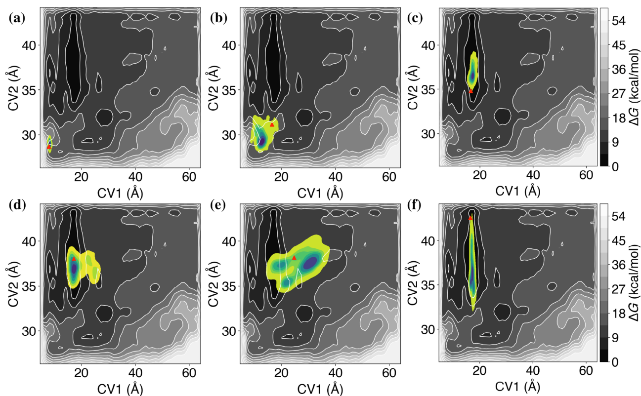
FIGURE 2 Probability densities of the CV values of the OCP-P3 domains separation. (a)–(f) Distributions of the CV1 and CV2 values obtained by unbiased equilibrium MD simulations. The distributions (colored) overlay the free energy surface of OCP-P3's domain separation (grey); dark colors denote relatively high probability densities. A red triangle denotes the coordinates (CV1, CV2) associated with the initial state used for the MD simulations. Each distribution was calculated from a set of four 100-ns simulations
