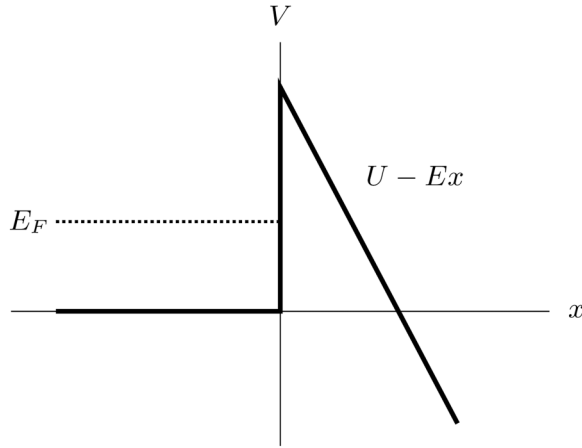
FIG. 1. The shape of the potential V(x) .
