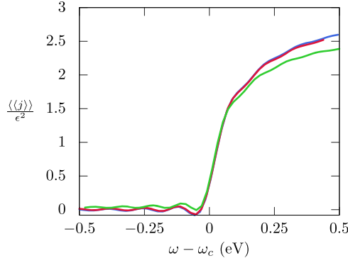
Figure 8. The average of the current \frac{1}{e^2} \langle \langle j \rangle \rangle after 12 periods as a function of \omega - \omega_c , for various values of the field: E = 3 \text{ Vnm}^{-1} (blue), E = 10 \text{ Vnm}^{-1} (red), E = 30 \text{ Vnm}^{-1} (green). We see a sharp transition as \omega crosses \omega_c .
