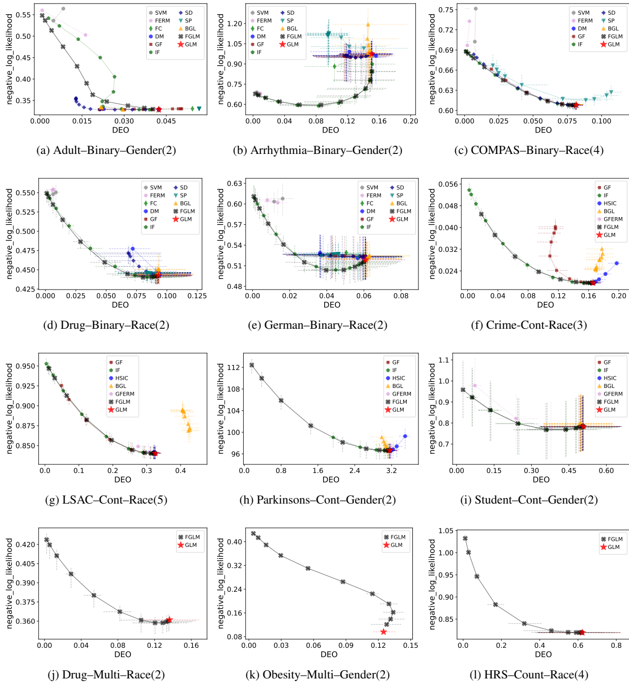
Figure 3. Experimental results in negative log-likelihoods and \mathcal{D}_{EO} from 11 real world datasets with binary (a-e) and continuous outcomes (f-i). Each subtitle is in the form of Dataset–Outcome Type–Sensitive Attribute( K ). For both binary and continuous outcomes we use a Generalized Linear Model (GLM, red star ★), Fair Generalized Linear Model (F-GLM, black X ✕), Individual Fairness penalty (IF, green pentagon ◈), Group Fairness penalty (GF, dark red square ■), and Bounded Group Loss (BGL, orange triangle ▲). Methods for binary outcomes also include the Support Vector Machine (SVM, grey hexagon ●), Fair Constraints (FC, green diamond ◆), Disparate Mistreatment (DM, blue circle ●), Squared Difference penalizer (SD, dark blue diamond ◆), Fair Empirical Risk Minimization (FERM, plum pentagon ◆), Statistical Parity (SP, teal triangle ▼). Methods for continuous outcomes include the HSIC penalty (HSIC, blue circle ●), General Fair Empirical Risk Minimization (GFERM, plum pentagon ◆). See Table 1 for additional information for each method. Each dot represents mean performance across test sets for a specific hyperparameter value \lambda .
