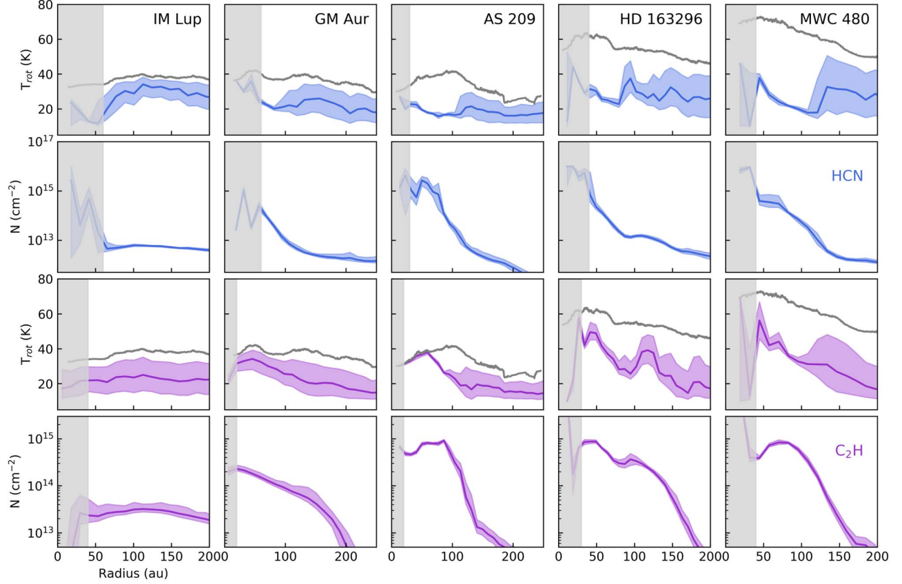
Figure B1. Best-fit rotational temperature and column density profiles to the 1–0 and 3–2 lines. The two upper and two bottom rows correspond to HCN and C 2 H, respectively. The gray curves correspond to the gas temperatures derived from the optically thick 12 CO 2–1 line (Law et al. 2021b) and was used as the maximum rotational temperature allowed in the fit. Gray shaded areas mark the regions where the lines are poorly fit. The resolution of the profiles is 0''3.
