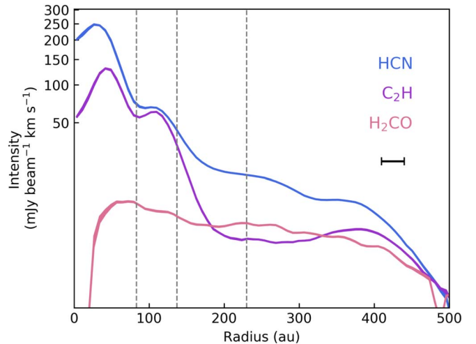
Figure 7. Deprojected radial profiles of the HCN, C 2 H, and H 2 CO 3–2 lines toward HD 163296. The profiles are computed from the tapered 0″.3 images. The dashed vertical lines mark the position of the putative planets at 83, 137, and 230 au (Teague et al. 2018a; Pinte et al. 2018b).
