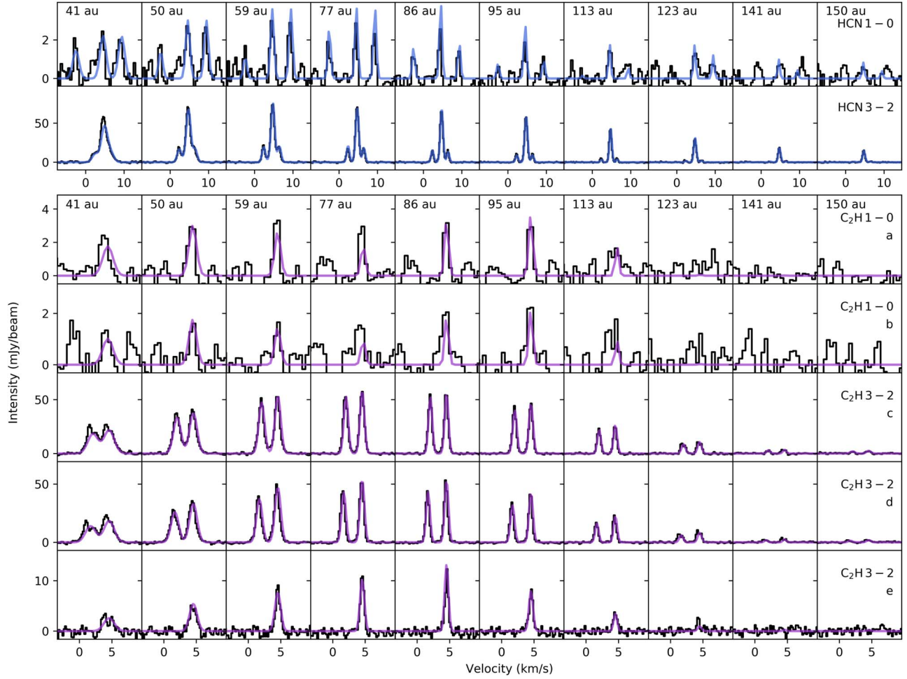
Figure B2. Deprojected spectra averaged over radial annuli in AS 209. HCN and \text{C}_2\text{H} lines are shown in the top and bottom panels, respectively. The 3–2 lines correspond to the tapered images with 0''.3 resolution. The observed spectra are shown in black, and the best-fit are shown in color. Several hyperfine lines are shown for \text{C}_2\text{H} : (a) and (b) correspond to the F = 2-1 and F = 1-0 components of the 1–0 line; (c) corresponds to the F = 4-3 and F = 3-2 components associated with the J = 7/2-5/2 group of the 3–2 line; (d) corresponds to the F = 3-2 and F = 2-1 components associated with the J = 5/2-3/2 group of the 3–2 line; and (e) corresponds to the F = 2-2 component associated with the J = 5/2-3/2 group of the 3–2 line.
