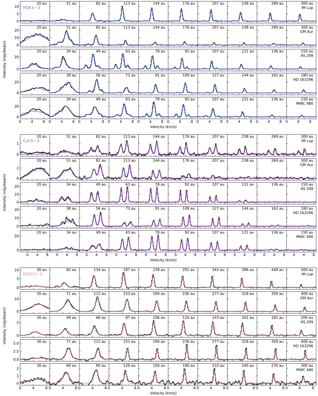
Figure 3. Deprojected spectra averaged over radial annuli for HCN (top), C 2 H (middle), and H 2 CO (bottom) lines. The observed spectra are shown in black, and the best-fit are shown in color. For H 2 CO, the best-fit model for a temperature of 20 K is shown. The radius of the center of each radial bin is shown at the top of each panel.
