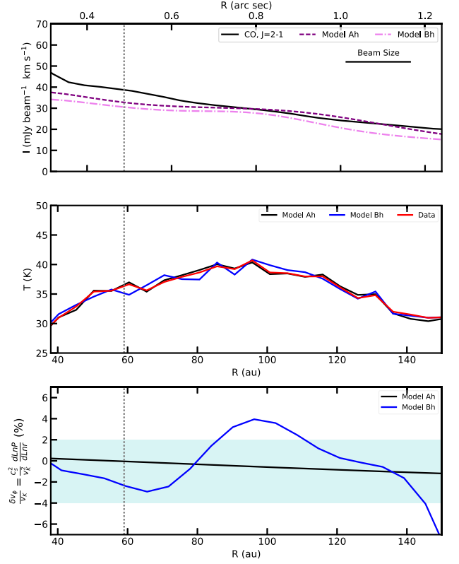
Figure 8. Comparison of data and expected values of thermochemical models with three iterations of hydrostatic equilibrium. Top: CO J=2-1 emission profile. Middle: thermal cuts for both models matching the brightness temperature of the CO J=2-1 line (Law et al. 2021a). Bottom: expected kinematic deviations in Models Ah and Bh with the range from the observations represented by the shaded area. The models show that the CO J=2-1 is, to a small uncertainty, well traced in both cases. The kinematic deviations in Models Ah and Bh show that even when a few iterations of hydrostatic equilibrium are considered, the results stand, i.e., the kinematic deviations in Model Bh with a H_2 gas depletion are stronger and cover a larger range than the ones observed in the data.
