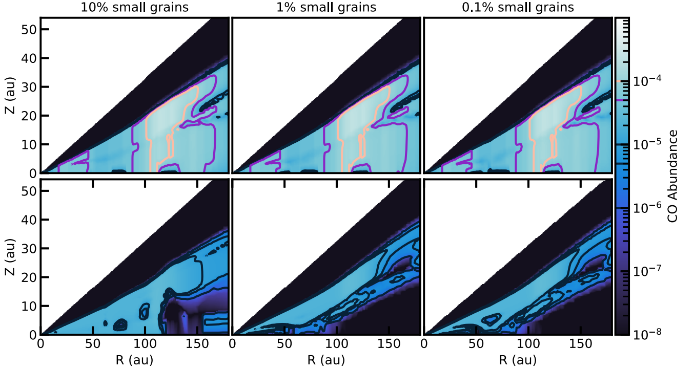
Figure 14. CO abundance structure for both model sets, A and B, with different localized depletion factors of small grains from left to right. Top row: CO abundance structure for Model A, where CO has been depleted and the gas surface density has a smooth profile. Bottom row: CO abundance structure for Model B, where CO is considered to trace the gas surface density by a constant scaling or CO/H 2 ratio. In both models, there are not significant changes with different degrees of small-grains depletion. However, we observe that in Model A, CO has a more uniform vertical distribution than in Model B.
