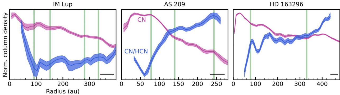
Figure 13. Normalized column density profiles of CN and CN/HCN (pink and blue lines, respectively), with NIR ring locations overplotted (green). NIR features are taken from Monnier et al. (2017), Avenhaus et al. (2018), and Rich et al. (2020). Horizontal black lines show the restoring beam FWHM of the line data.
