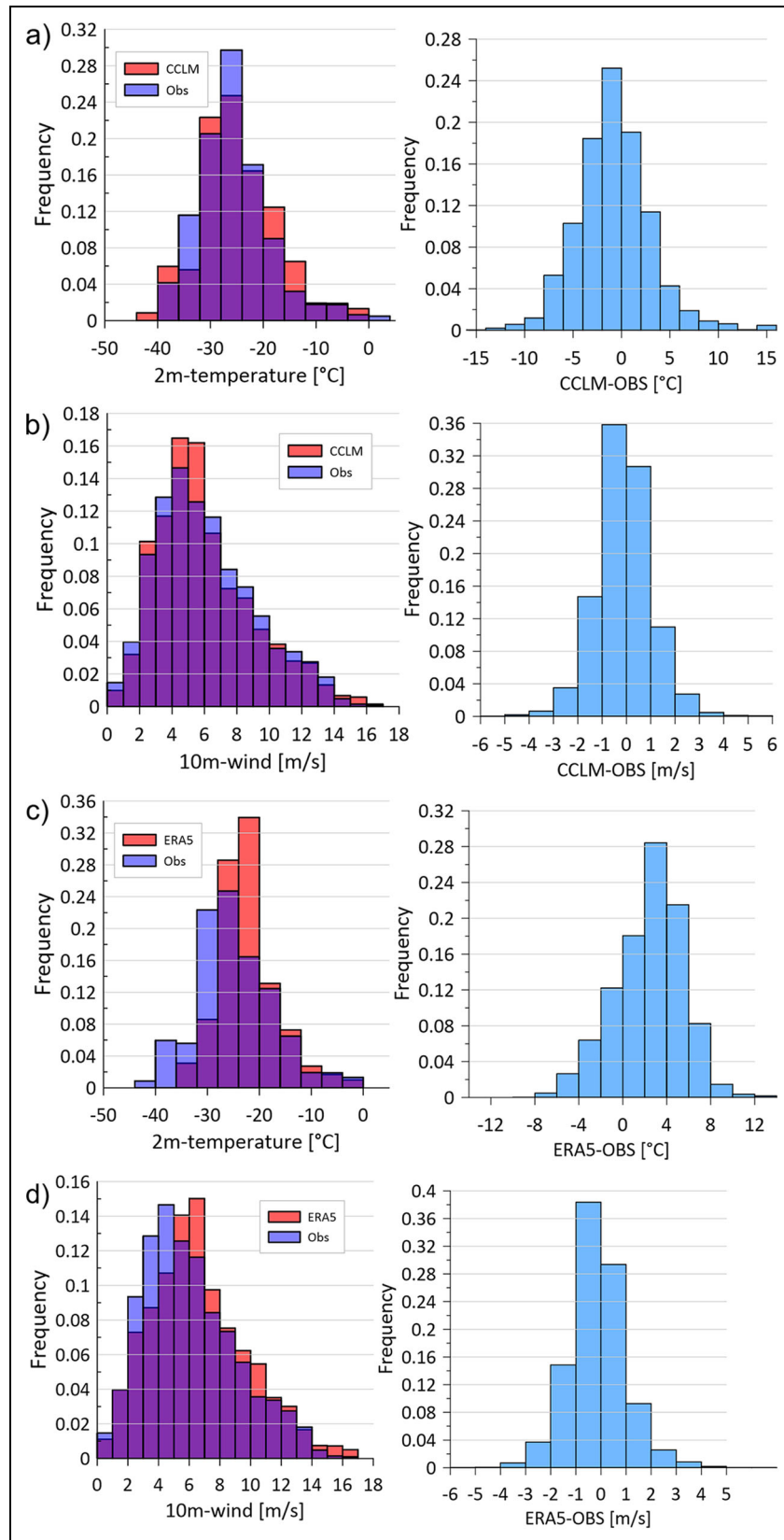
Figure 12. Frequency distributions of tower measurements and simulations for wind and temperature. Frequency distributions of measured (tower) and simulated values (1 h values) and their differences for C15MOD0 (a, b) and ERA5 (c, d) for November 2019 to April 2020: (a/c) 2-m temperature, (b/d) 10-m wind speed.
