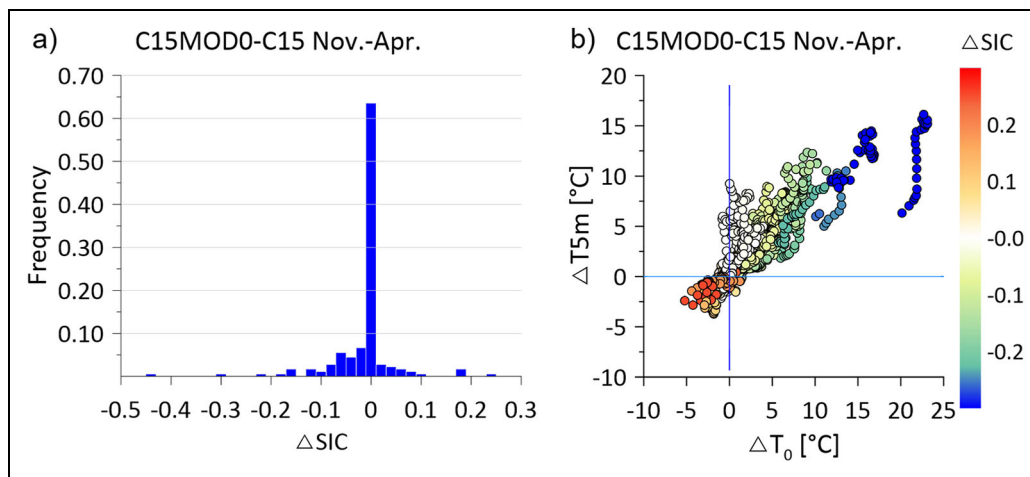
Figure 19. Frequency distribution of SIC differences and scatter plot of IST and air temperature differences for the grid point of Polarstern. (a) Frequency distribution of the SIC differences between the C15Mod0 and the C15 run (bins of 0.02). (b) Scatter plot of IST and 5-m temperature differences between the C15MOD0 and the C15 run (hourly data, SIC difference color coded).
