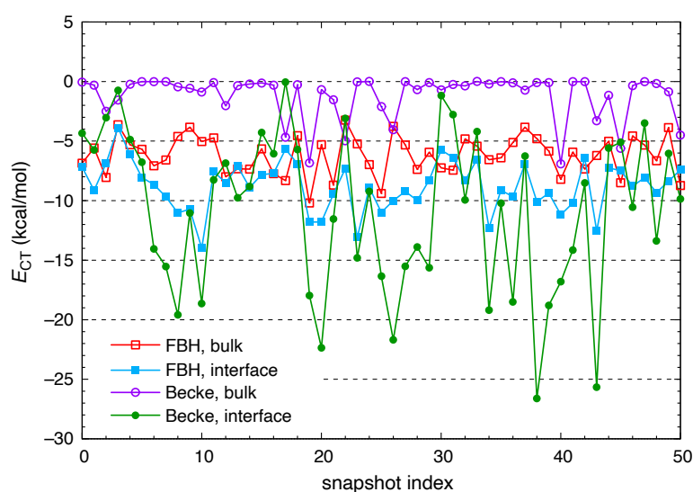
Figure 4. CT energies for \text{ClO}^-(\text{aq}) , computed using either Becke partition or else FBH weighting to define the CT-free reference state, and considering both the bulk and interfacial data sets.
