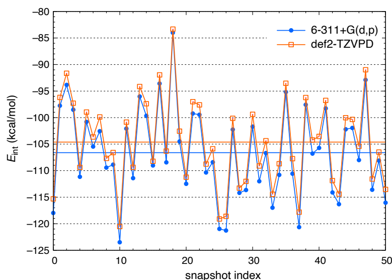
Figure 1. Total interaction energies for snapshots of \text{Cl}^- (\text{aq}) in bulk water, computed at the SAPT0 + MBD level using two different basis sets. Solid horizontal lines show the ensemble-averaged values obtained using either basis set. These averages are \langle E_{\text{int}} \rangle = -106.6 \pm 8.4 kcal/mol for 6-311+G(d,p) and \langle E_{\text{int}} \rangle = -104.6 \pm 8.2 kcal/mol for def2-TZVPD, where the uncertainties represent one standard deviation.
