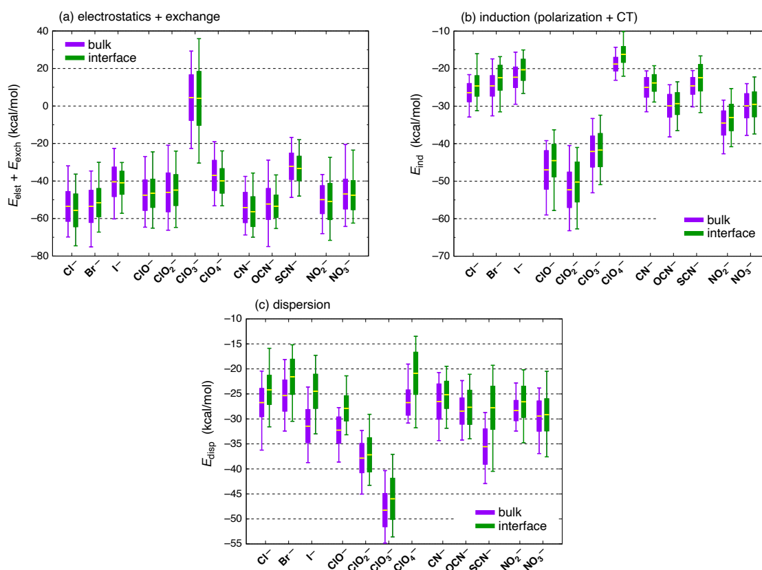
Figure 7. Box-and-whisker plots showing mean values, standard deviations, and extremal values of ion–water interaction energy components computed at the SAPT0 + MBD/6-311+G(d,p) level: (a) first-order electrostatics and exchange, E_{\text{elst}} + E_{\text{exch}} ; (b) E_{\text{ind}} from Equation (5); and (c) E_{\text{disp}} from the MBD model. The sum of the energy components in panels (a–c) equals E_{\text{int}} in Figure 5a.
